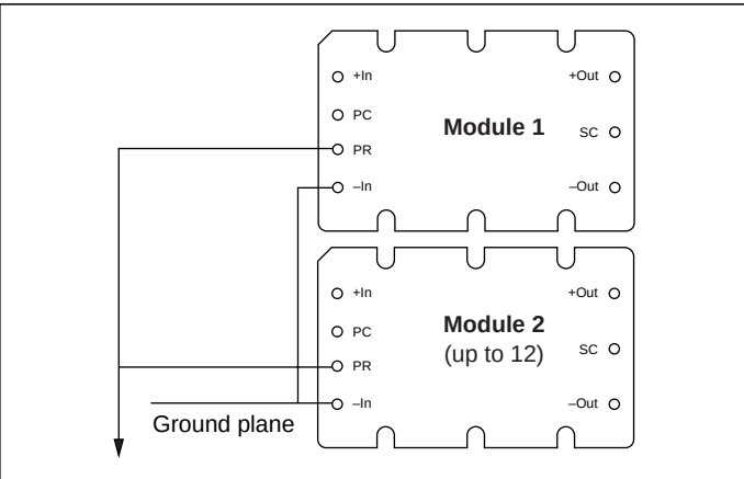
Figure 9—DC coupled single-wire interface.
