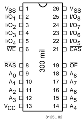
26/24 Lead SOJ PIN CONFIGURATION Top View
