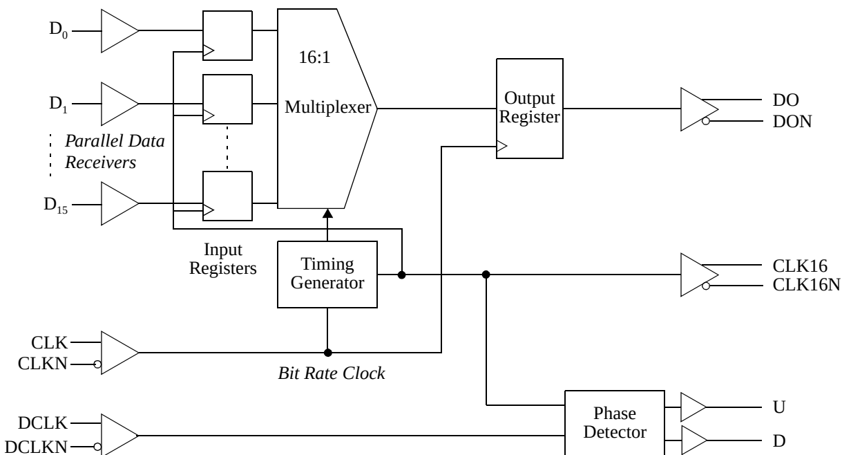
Figure 2: VS8062 Block Diagram
