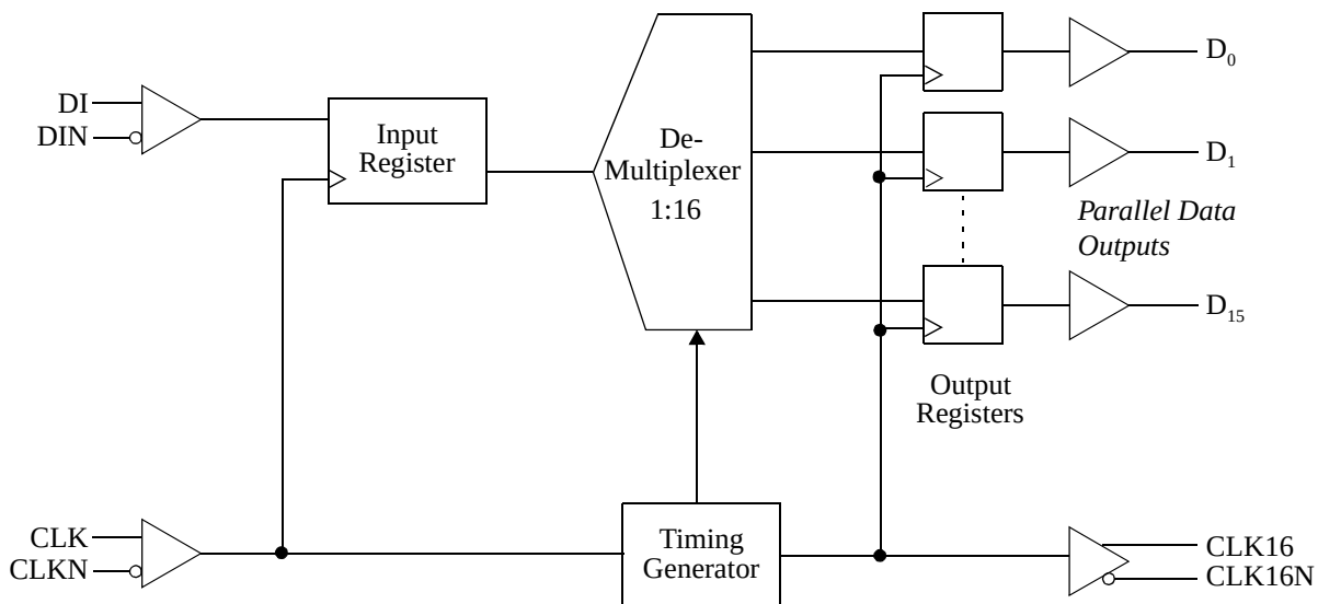
Figure 2: VS8062 Block Diagram
