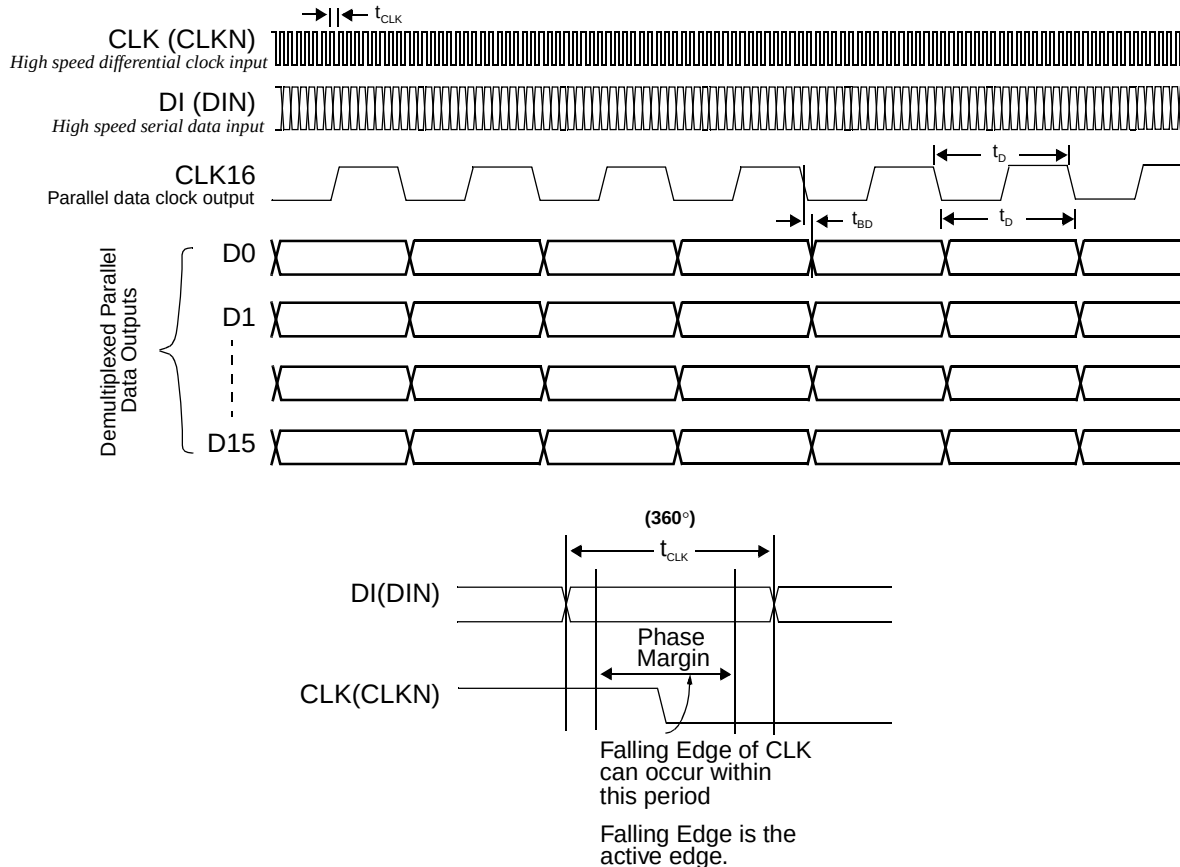
Figure 6: VS8062 Timing Diagram
