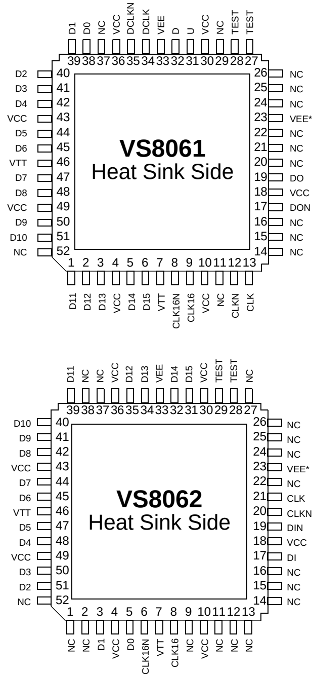
Figure 9: VS8061/8062 F (52-Pin LDCC) Pin Diagrams
