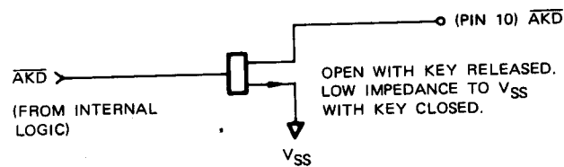
Figure 5. \overline{\text{AKD}} Output Structure
