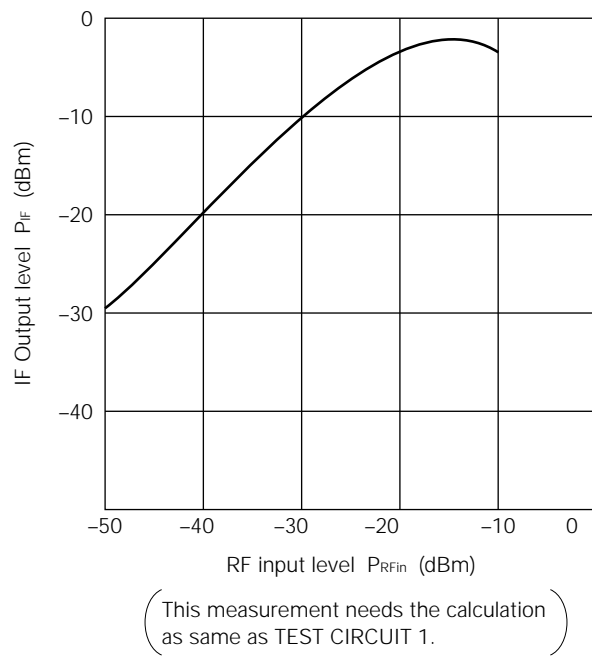
RF input level vs. IF output level
