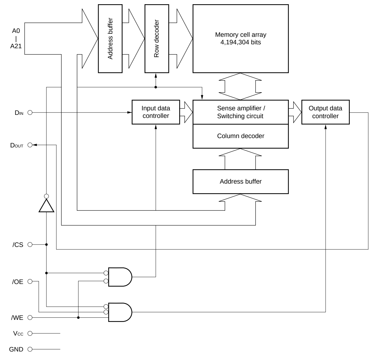
Block Diagram
