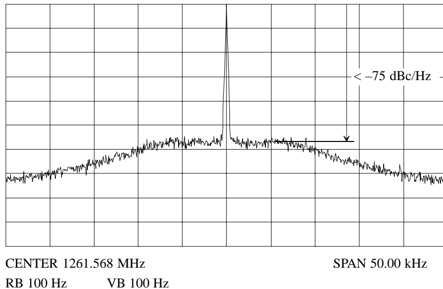
Figure 7. Phase noise
