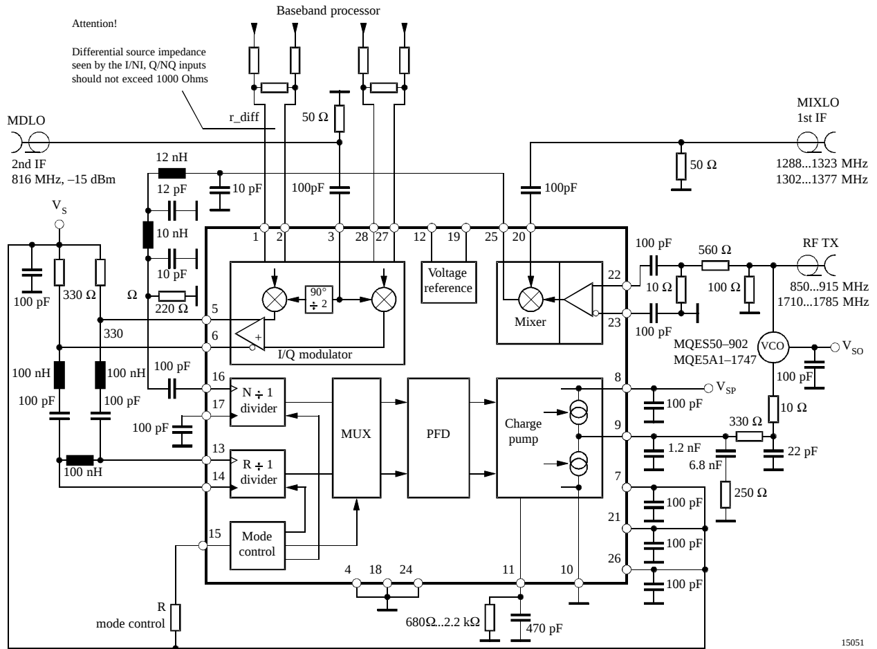
Figure 16. Application circuit (power-up and 680 \Omega to 2.2 k \Omega charge-pump control is not shown)
