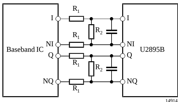
Figure 13. Interfacing the U2895B to I/Q baseband circuits
