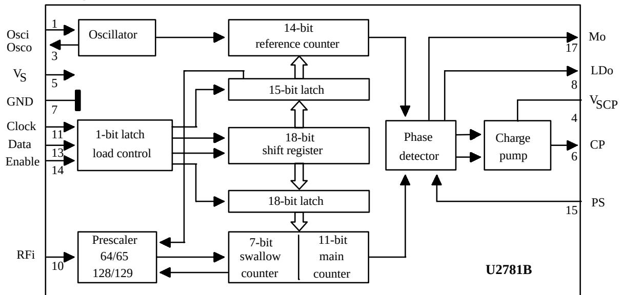
Figure 1. Block diagram
