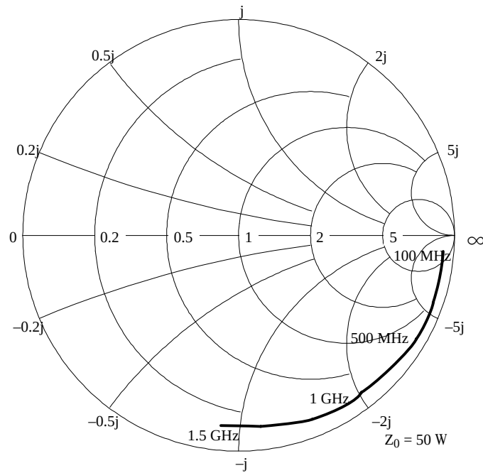
Figure 8. Input impedance
