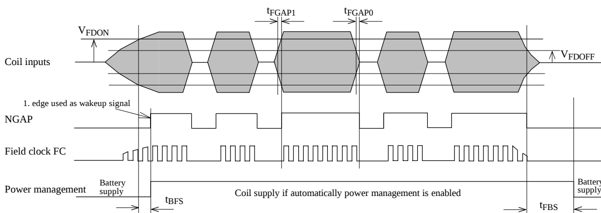
Figure 4. Modulation
