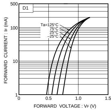
Fig.5 Forward characteristics
