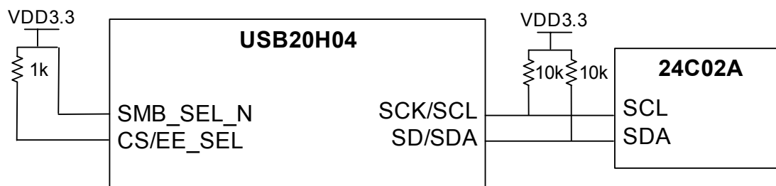
Figure 8.1 - 2-Wire EEPROM Interface
