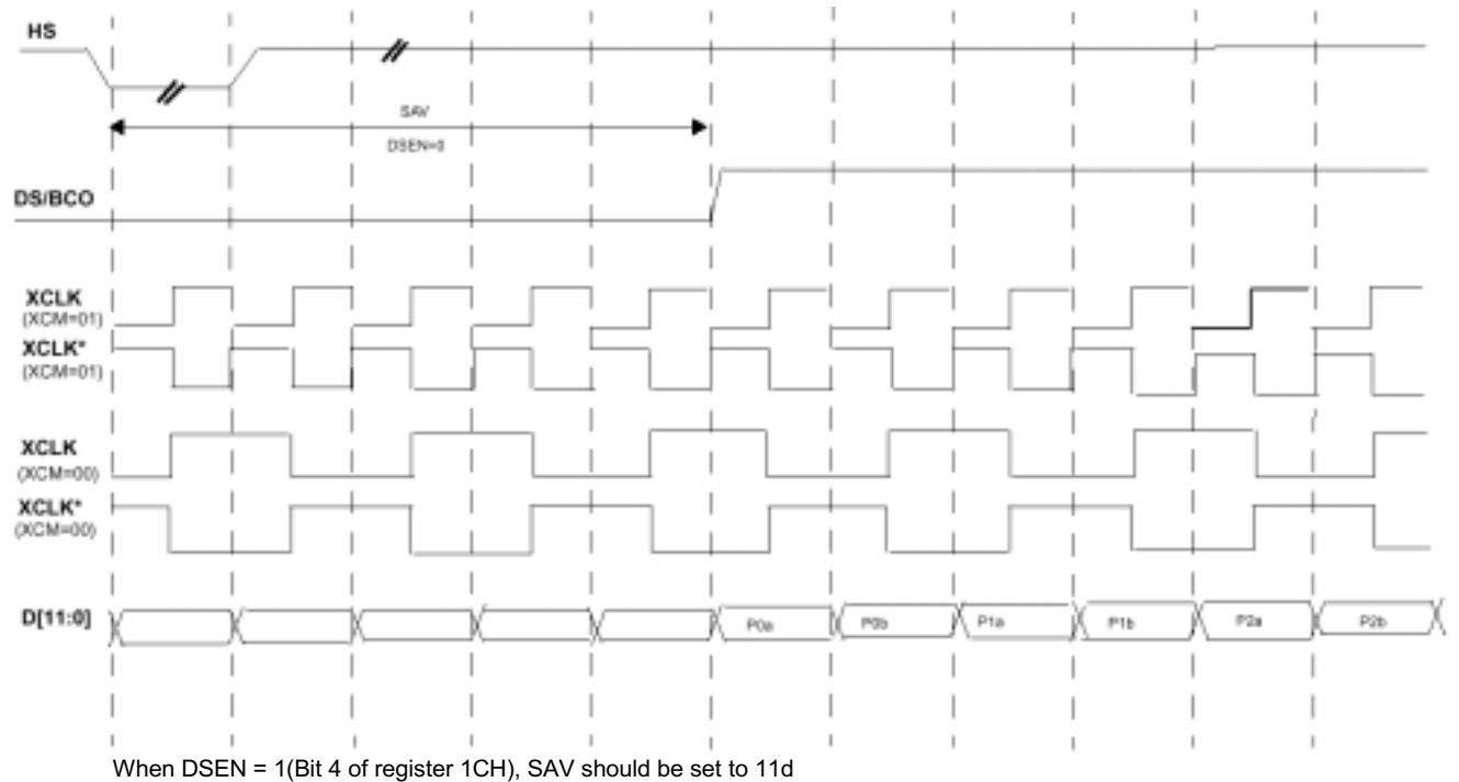
Figure 1-3. Non-multiplexed Data Transfers
