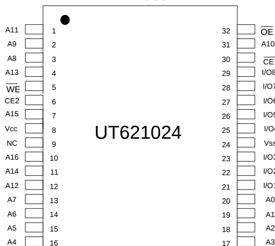
PDIP / SOP
