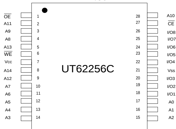
PDIP/SOP
