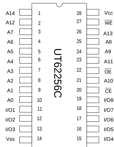
PDIP/SOP
