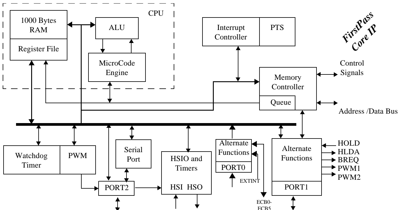
Figure 1. UT80CRH196KD Microcontroller
