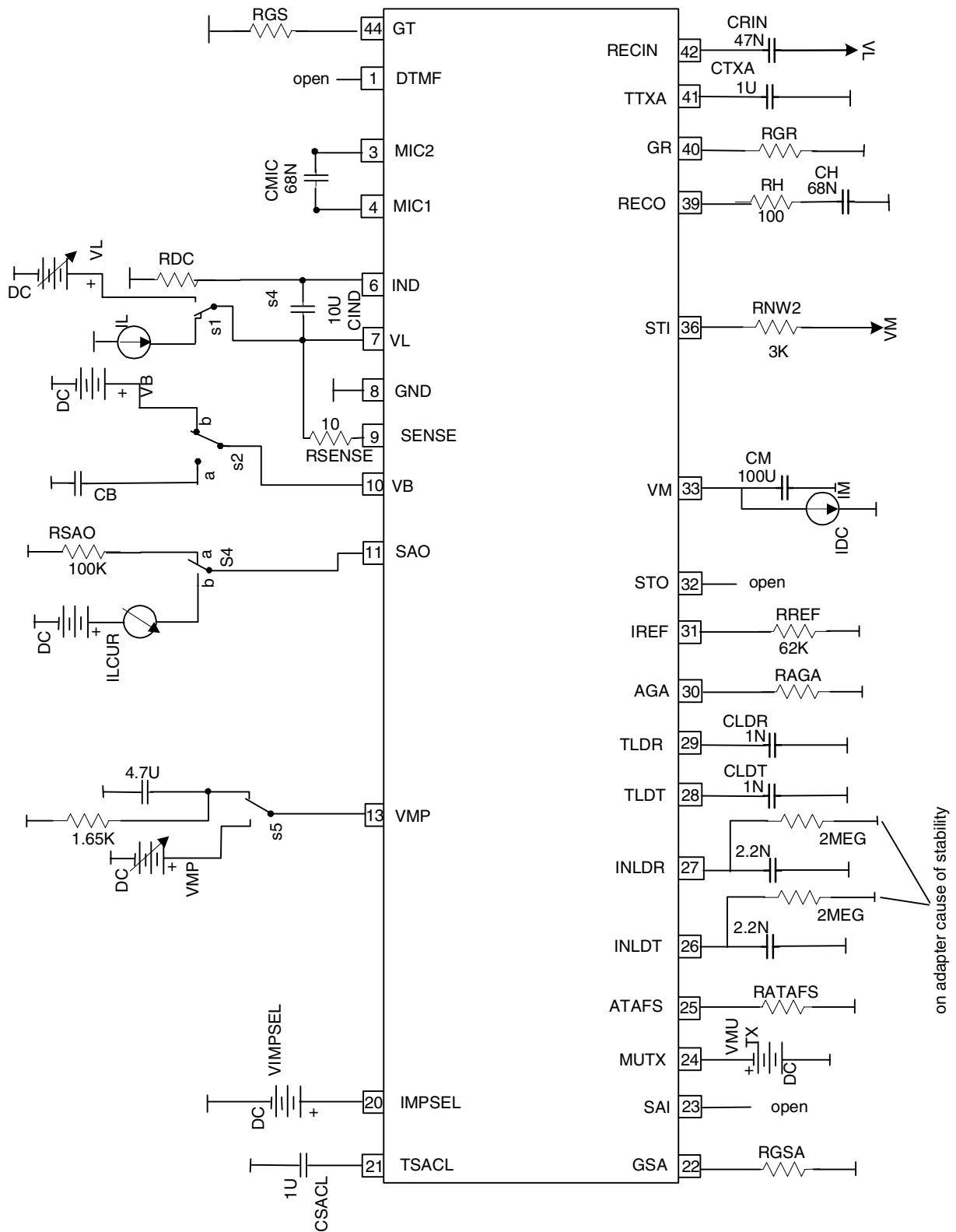
Figure 22. AC Tests
