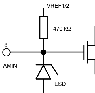
Figure 8. Internal Circuit at Pin AMIN
