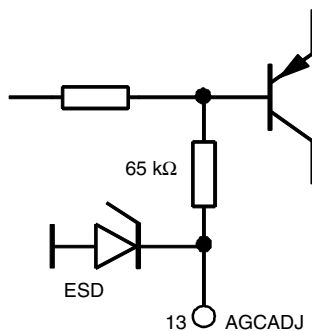
Figure 6. Internal Circuit at Pin AGCADJ
