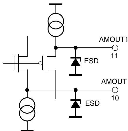
Figure 9. Internal Circuit at Pins AMOUT1 and AMOUT
