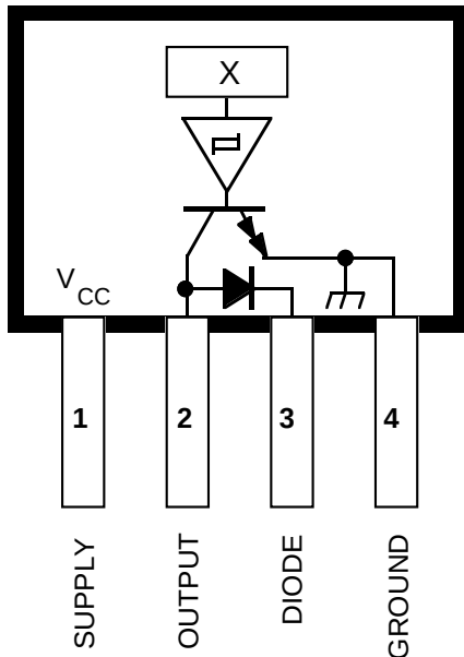
Dwg. PH-001
