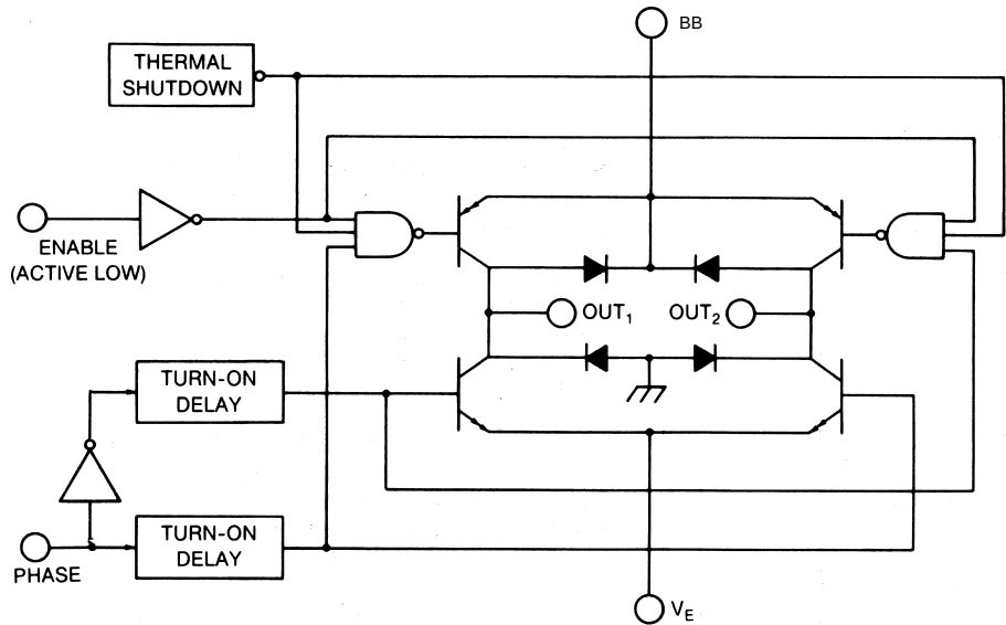
FUNCTIONAL BLOCK DIAGRAM (ONE OF TWO DRIVERS)
