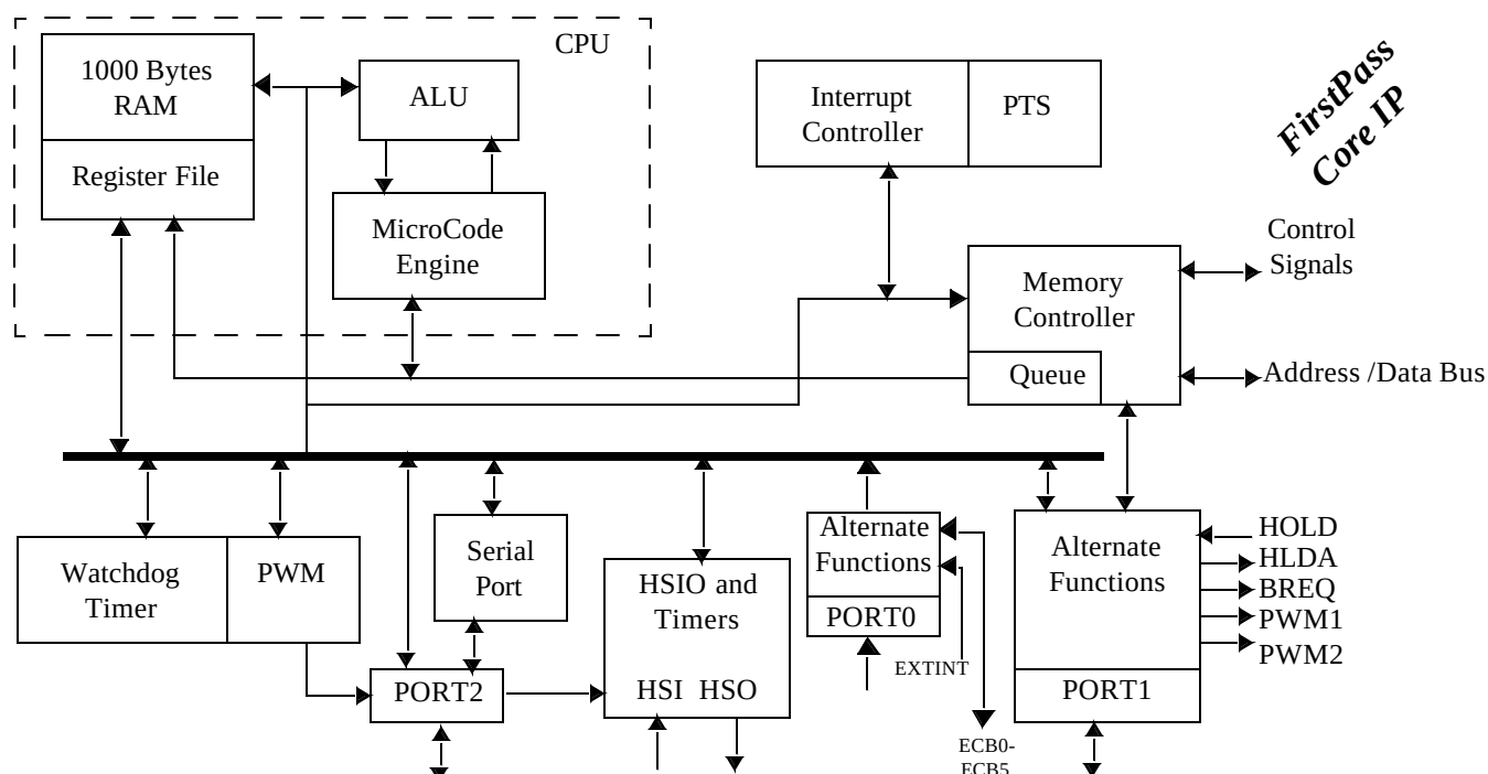
Figure 1. UT80C196KDS Microcontroller
