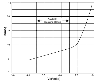
Fig 15 Supply Current vs Supply Voltage
