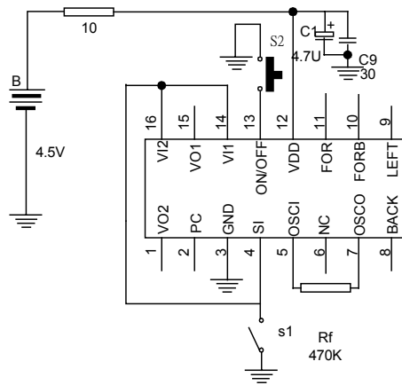
Figure2 Testing stand-by current
