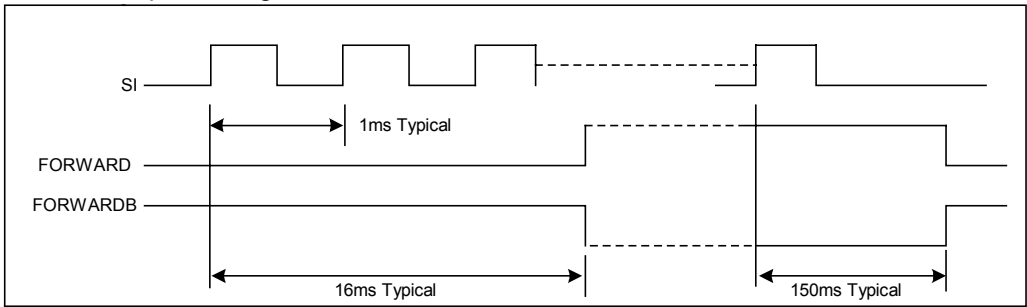
Forward Output Timing
