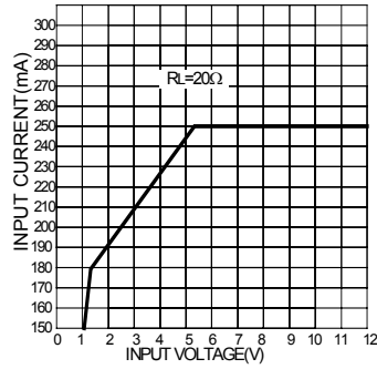
Fig.5 Input Current
