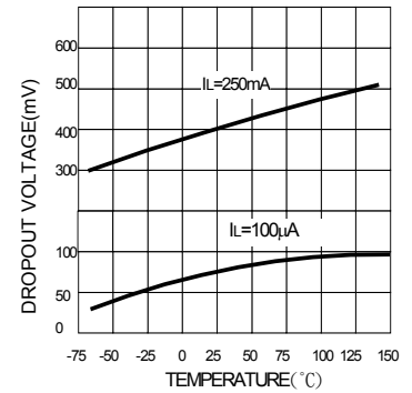
Fig. 6 Dropout Voltage
