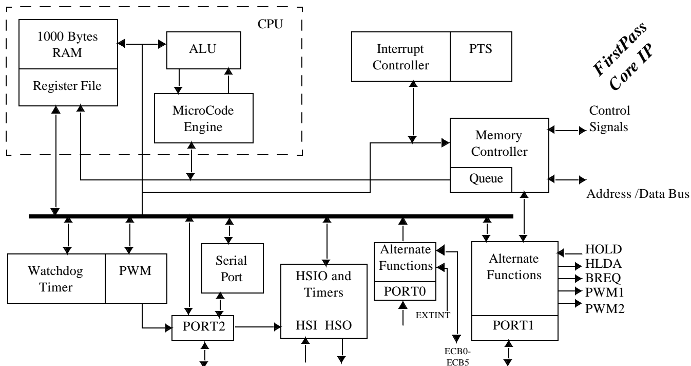
Figure 1. UT80C196KD Microcontroller
