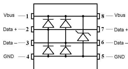
PAD LAYOUT
