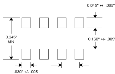
PAD LAYOUT
