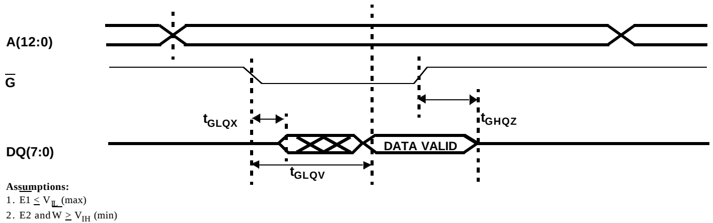
Figure 3c. SRAM Read Cycle 3: Output Enable Access
