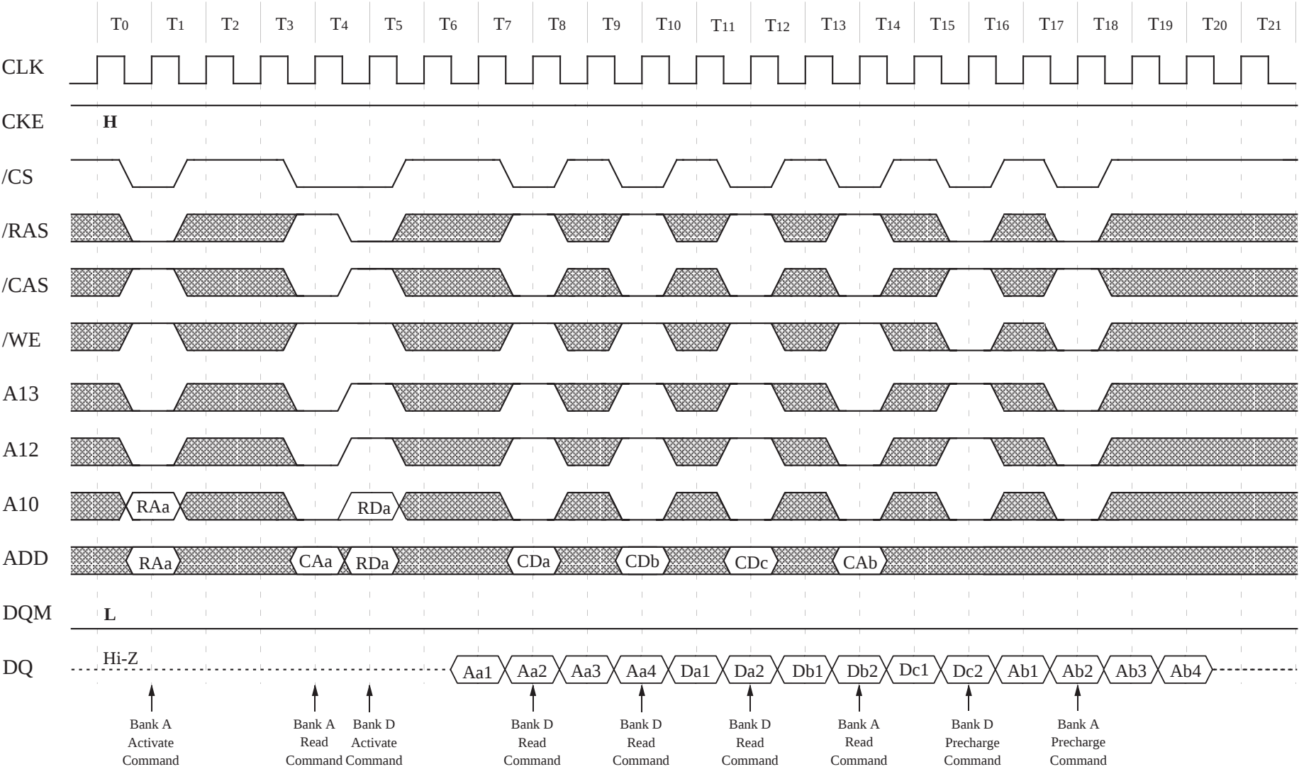
Interleaved Column Read Cycle (2/2) (Burst length = 4, /CAS latency = 3)
