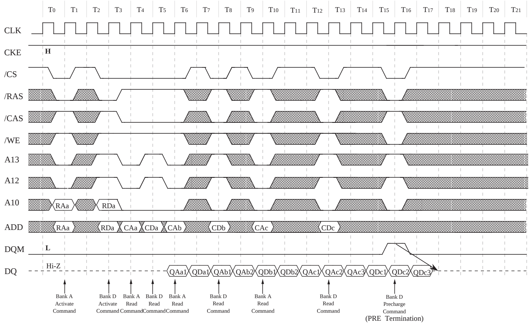
13.25 Full Page Random Column Read (Burst length = Full Page, /CAS latency = 2)
