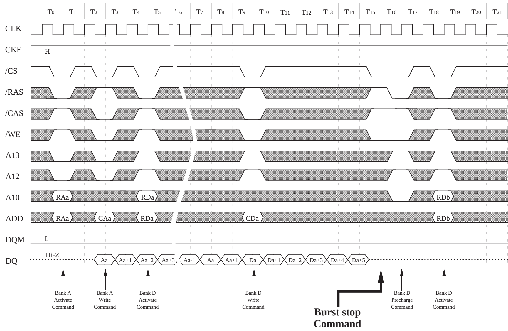
13.22 Full Page Write Cycle (1/2) (/CAS latency = 2)
