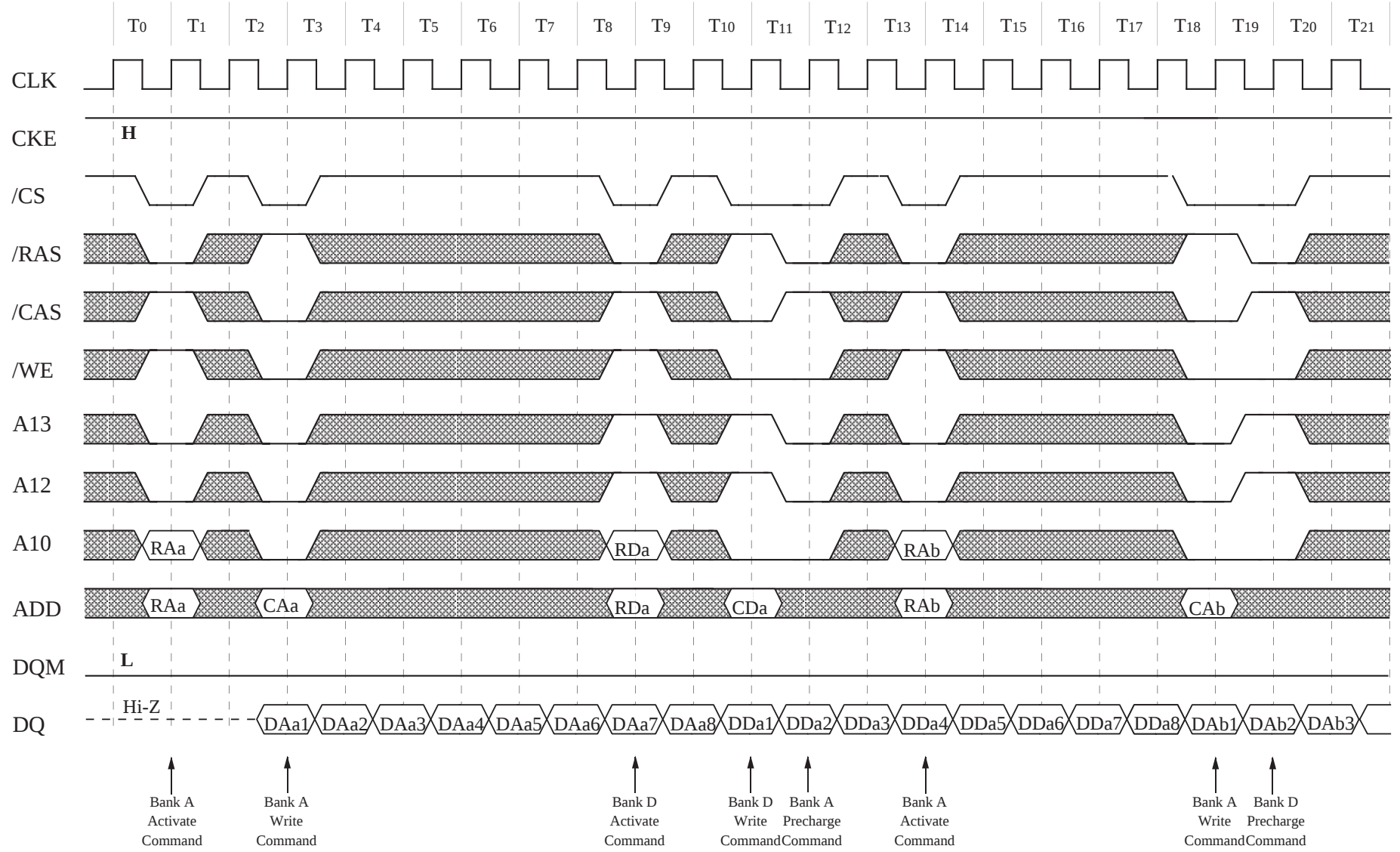
13.15 Random Row Write (Ping-Pong banks) (1/2) (Burst length = 8, /CAS latency = 2)
