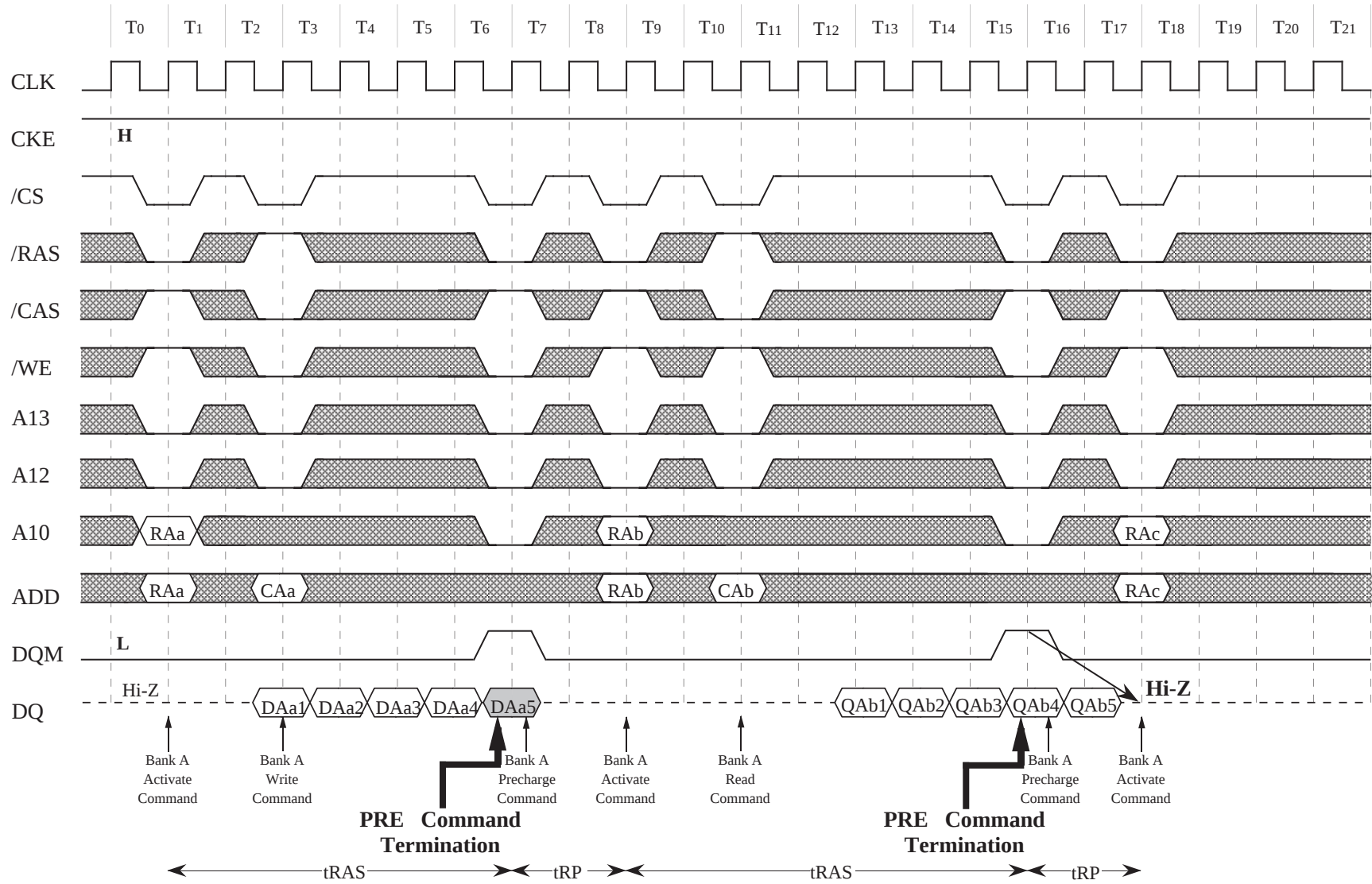
13.27 PRE (Precharge) Termination of Burst (1/2) (Burst length = 8, /CAS latency = 2)
