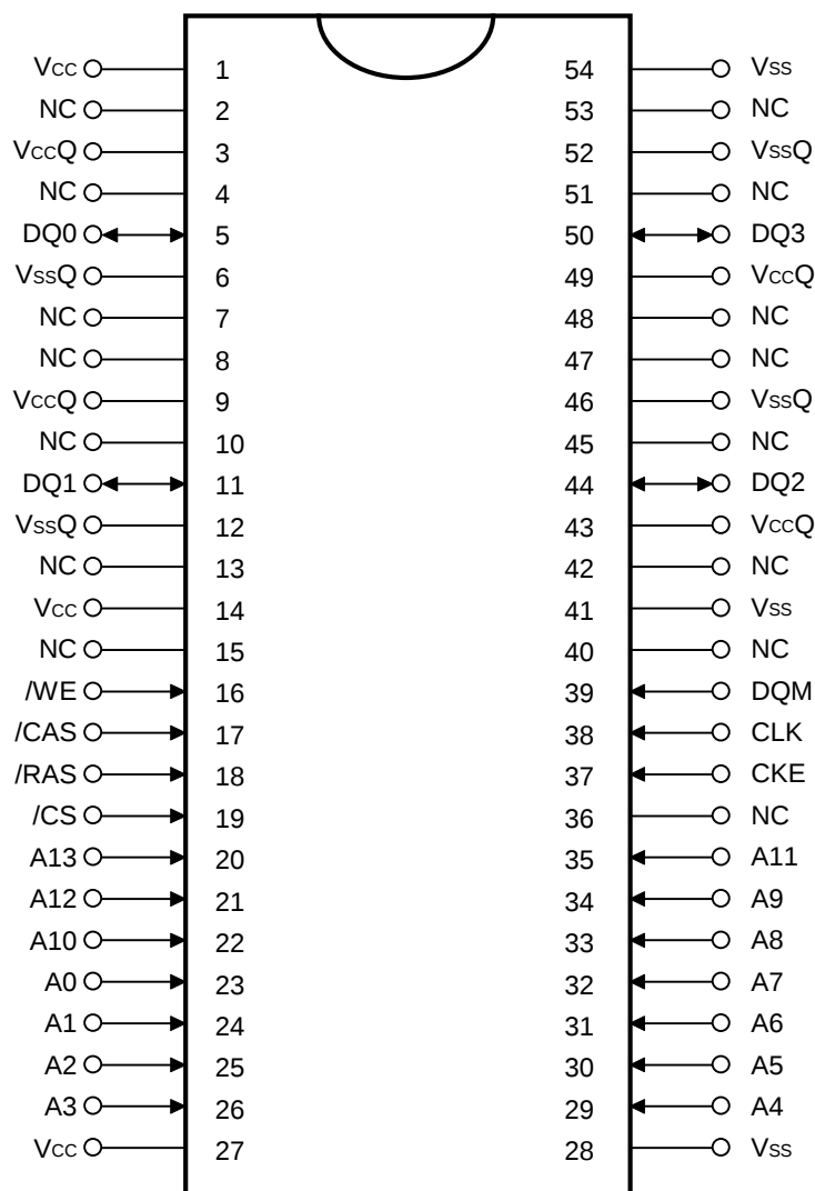
54-pin Plastic TSOP(II) (400mil) 4M words x 4 bits x 4 banks
