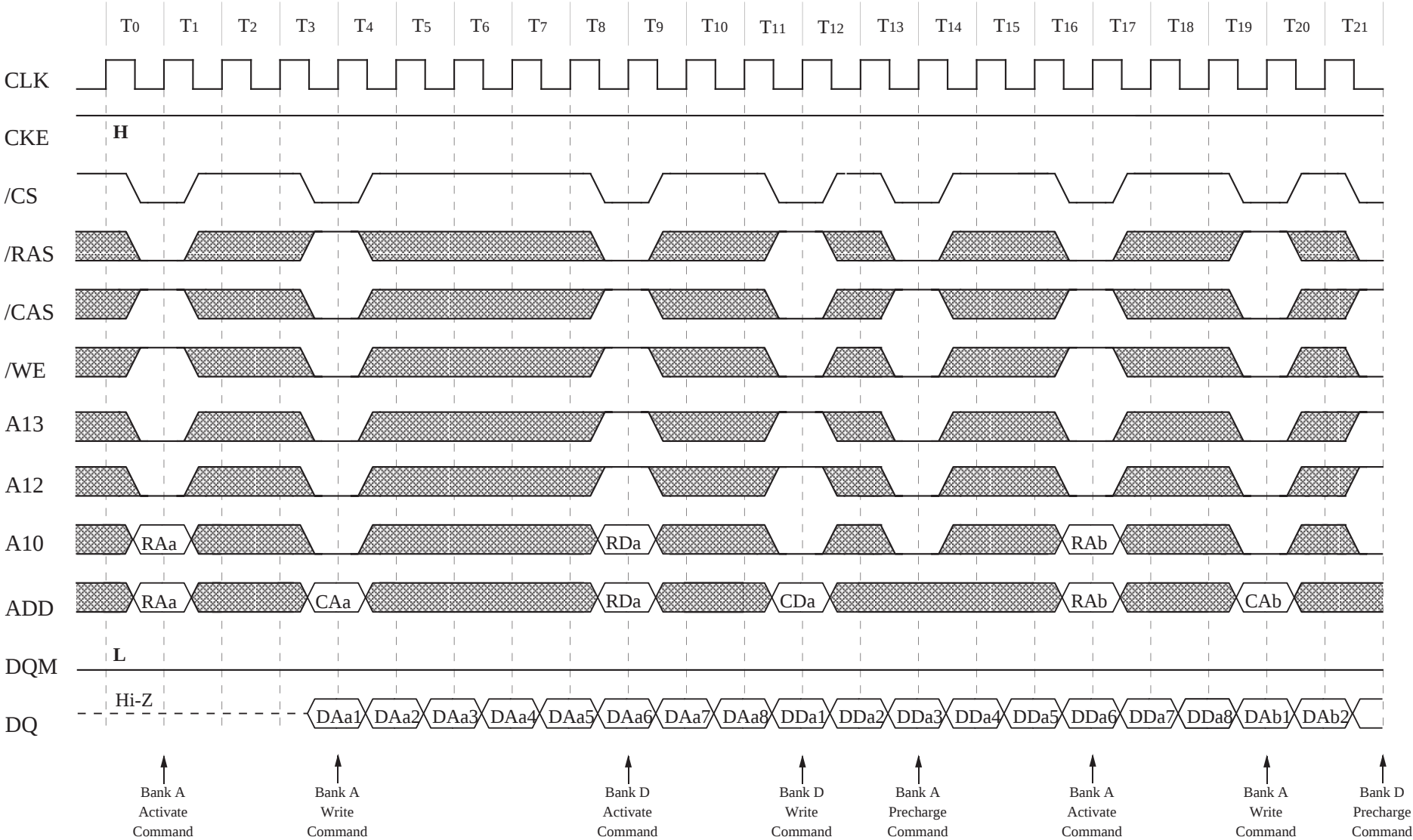
Random Row Write (Ping-Pong banks) (2/2) (Burst length = 8, /CAS latency = 3)
