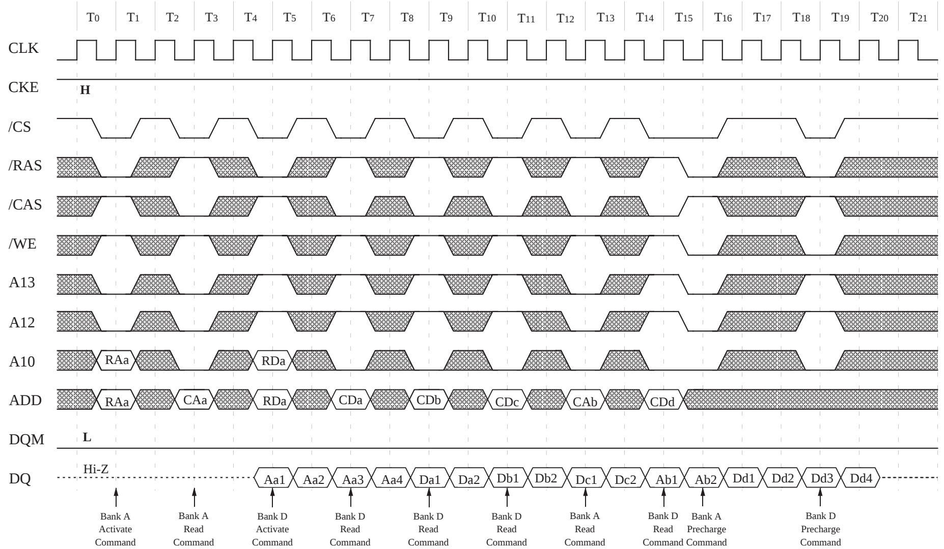
13.17 Interleaved Column Read Cycle (1/2) (Burst length = 4, /CAS latency = 2)
