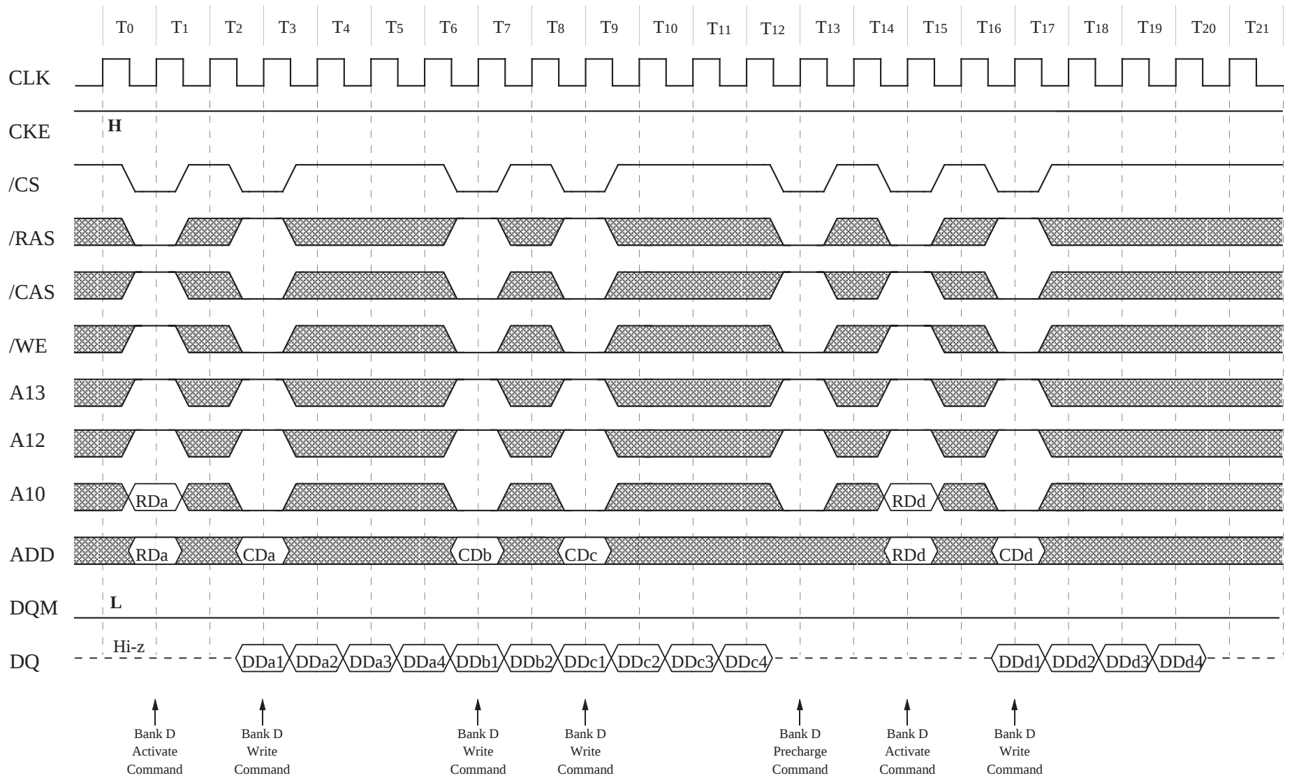
13.13 Random Column Write (Page with same bank) (1/2) (Burst length = 4, /CAS latency = 2)
