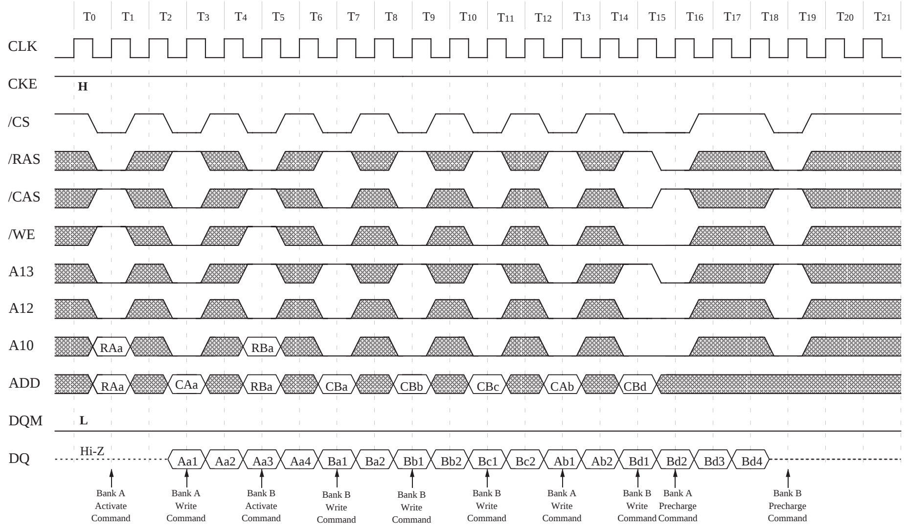
13.18 Interleaved Column Write Cycle (1/2) (Burst length = 4, /CAS latency = 2)
