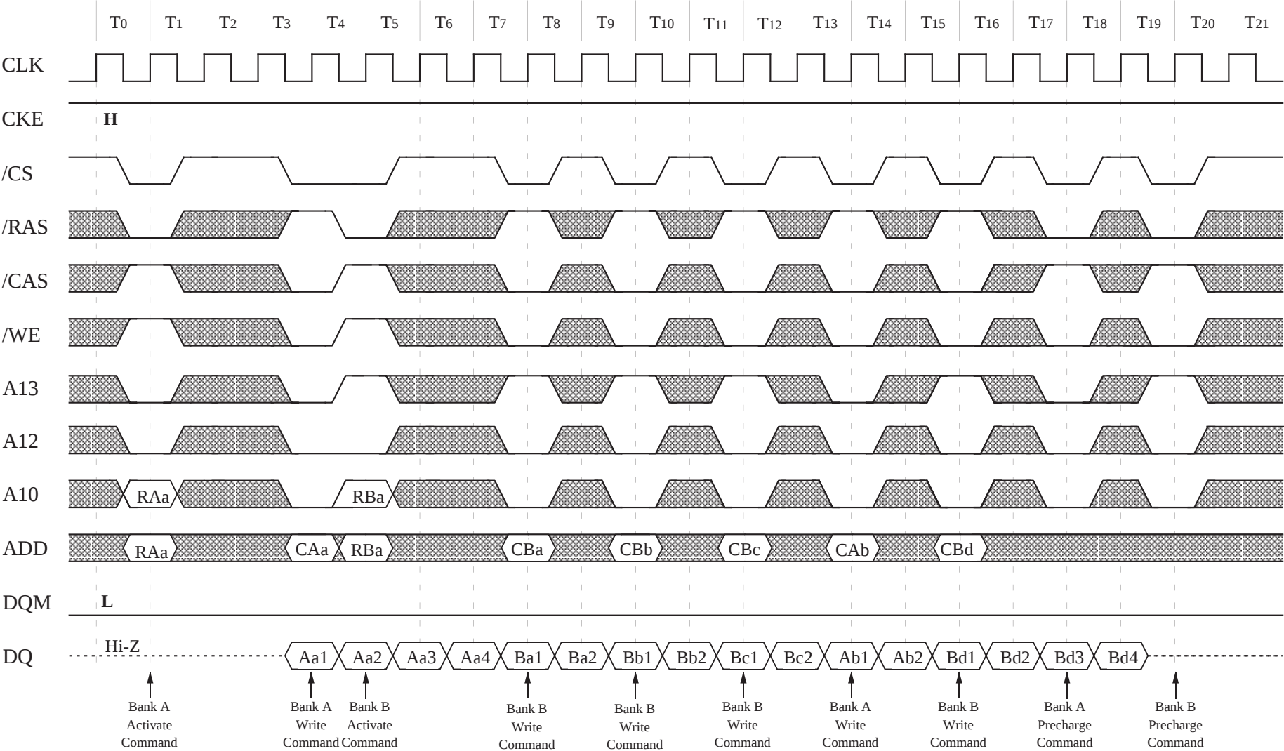
Interleaved Column Write Cycle (2/2) (Burst length = 4, /CAS latency = 3)
