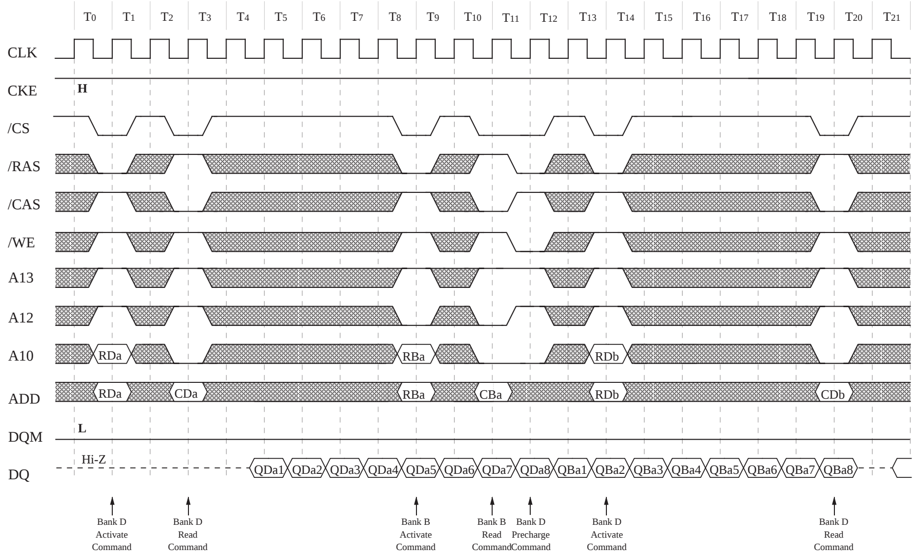
13.14 Random Row Read (Ping-Pong banks) (1/2) (Burst length = 8, /CAS latency = 2)
