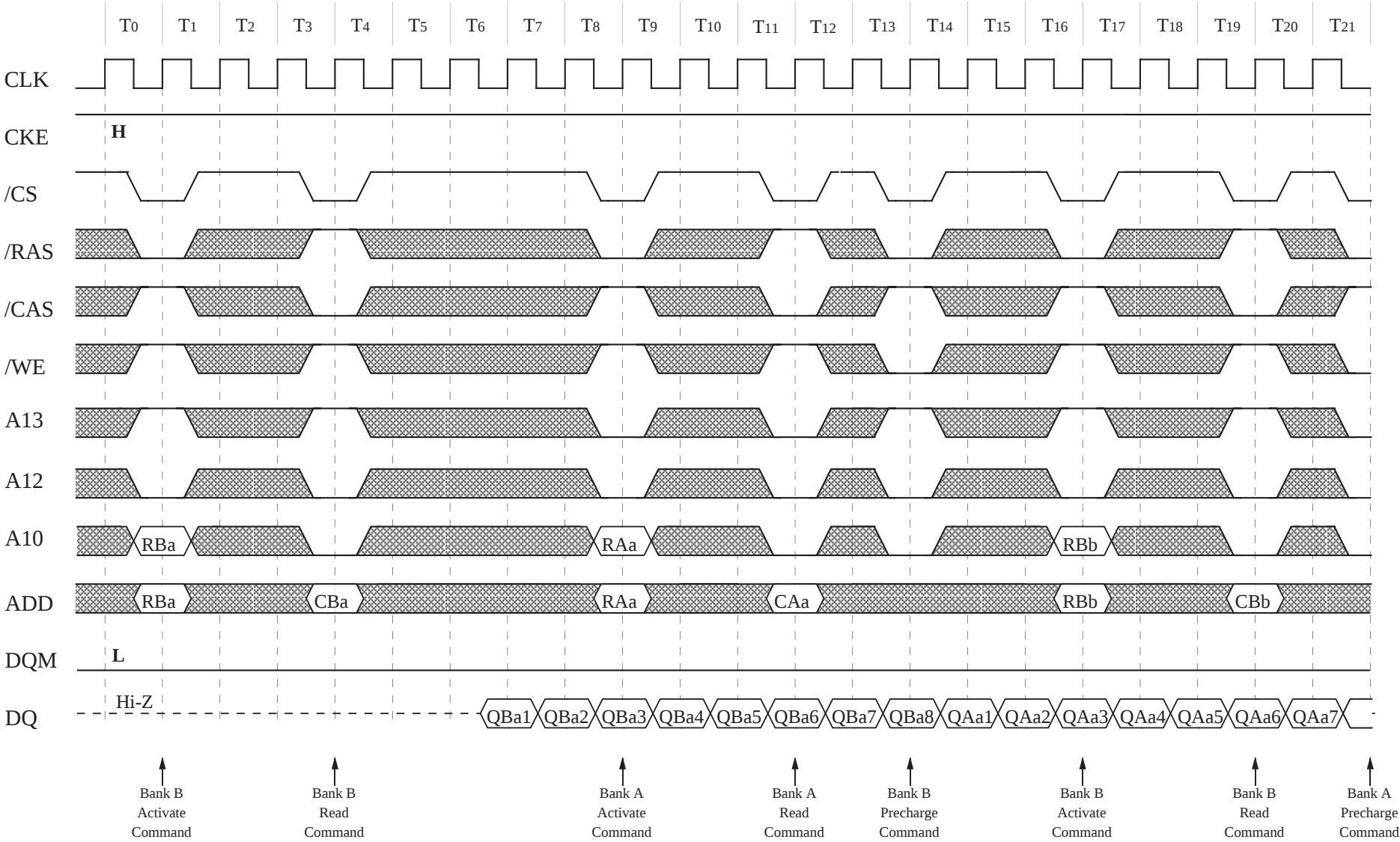
Random Row Read (Ping-Pong banks) (2/2) (Burst length = 8, /CAS latency = 3)
