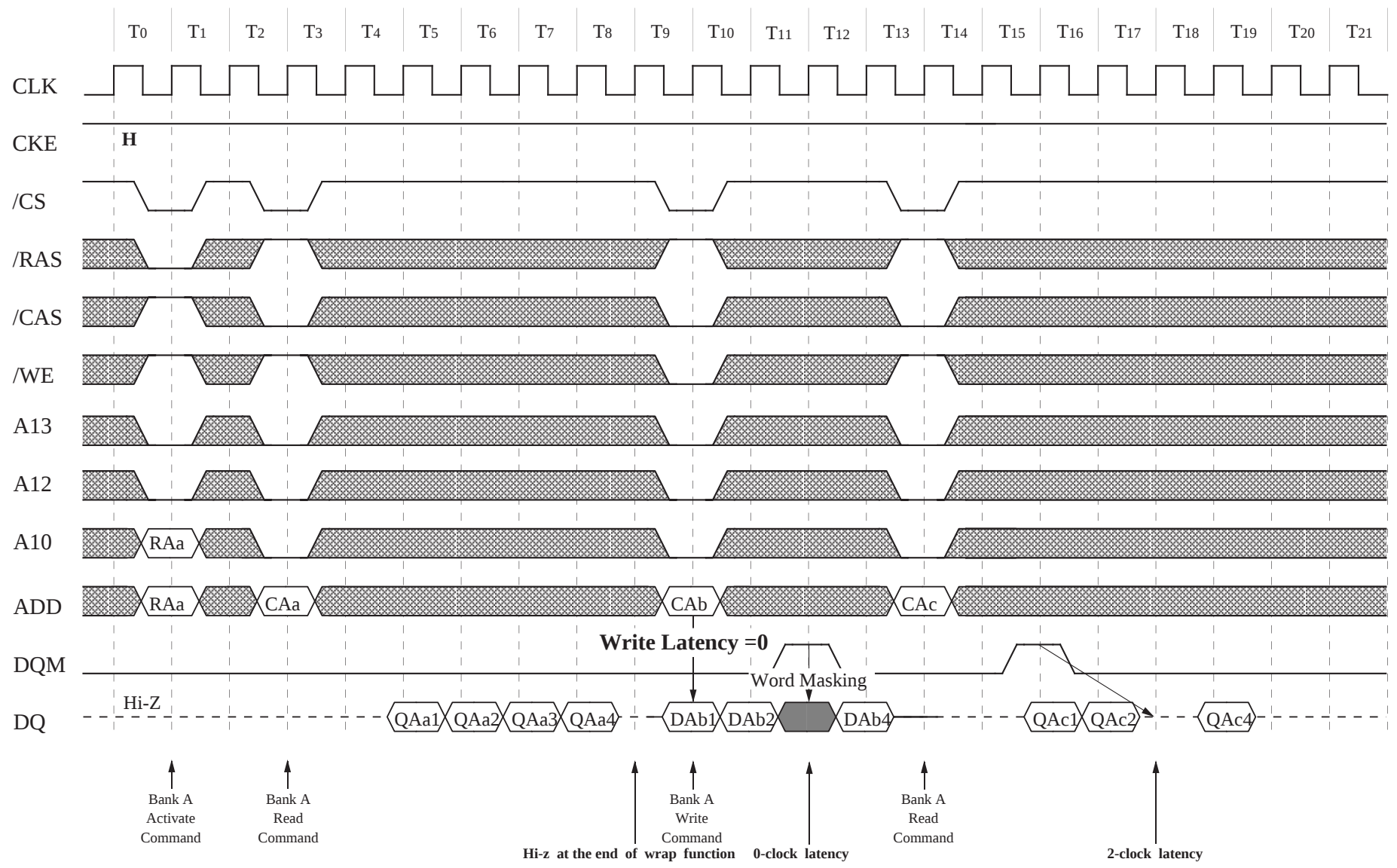
13.16 Read and Write (1/2) (Burst length = 4, /CAS latency = 2)
