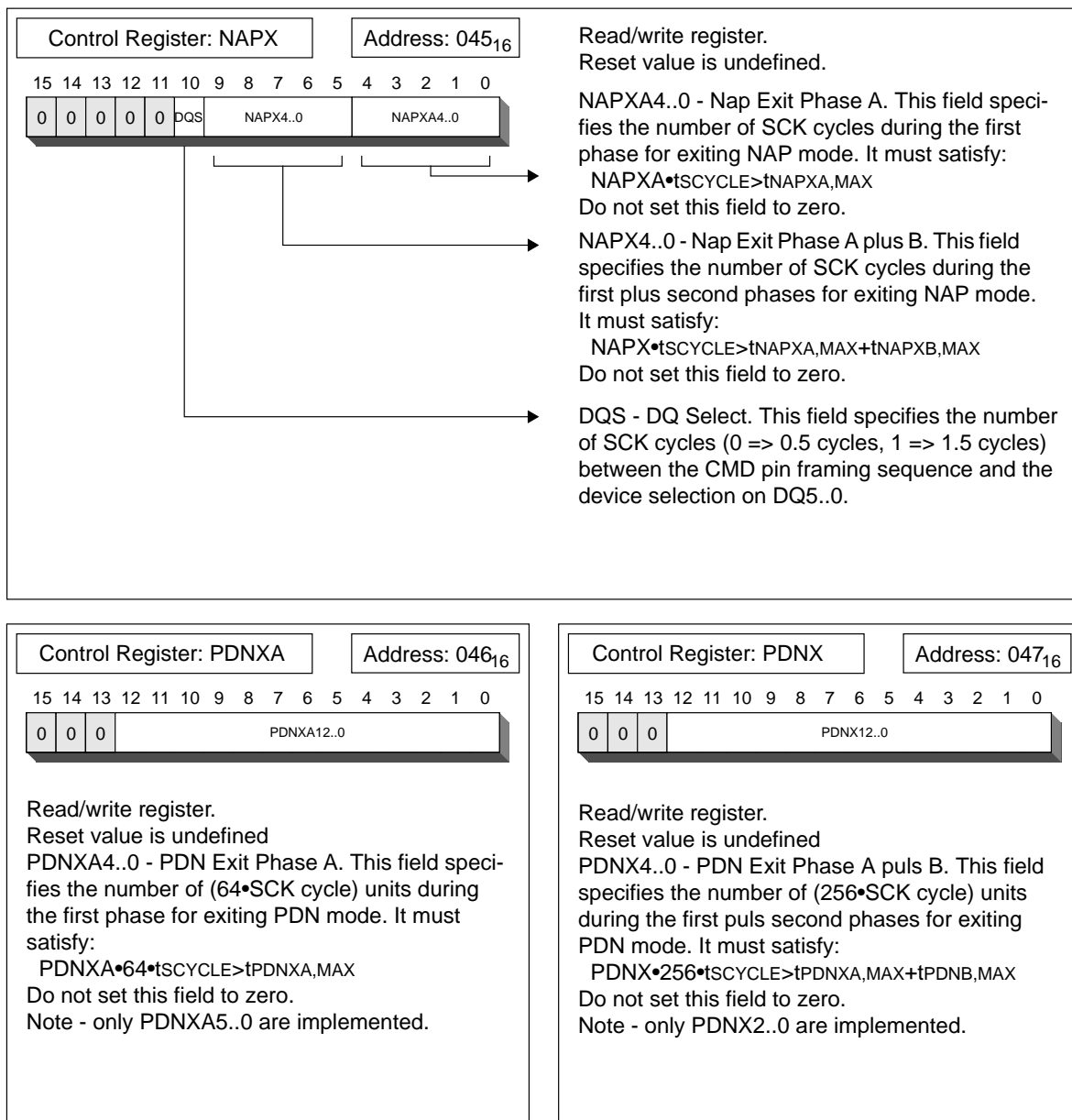
Figure 22-1 Control Registers (4/6)
