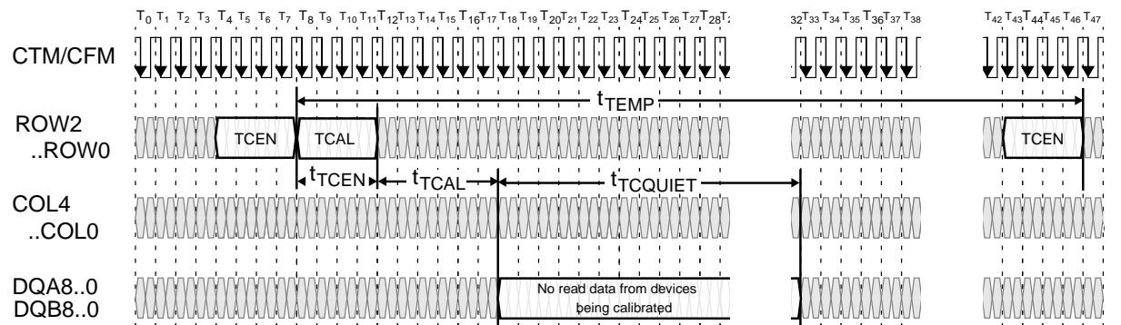
Figure 25-2 Temperature Calibration (TCEN-TCAL) Transactions to RDRAM
