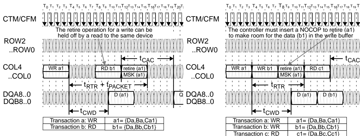
Figure 15-2 Retire Held Off by Read (left) and Controller Forces WWR Gap (right)
