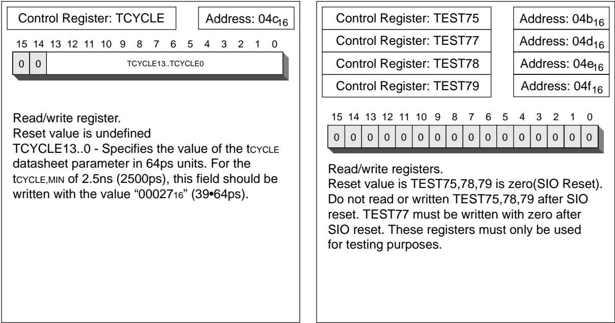
Figure 22-1 Control Registers (6/6)
