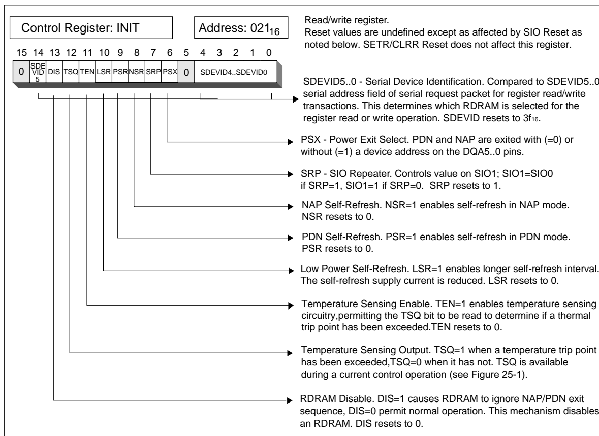
Figure 22-1 Control Registers (1/6)
