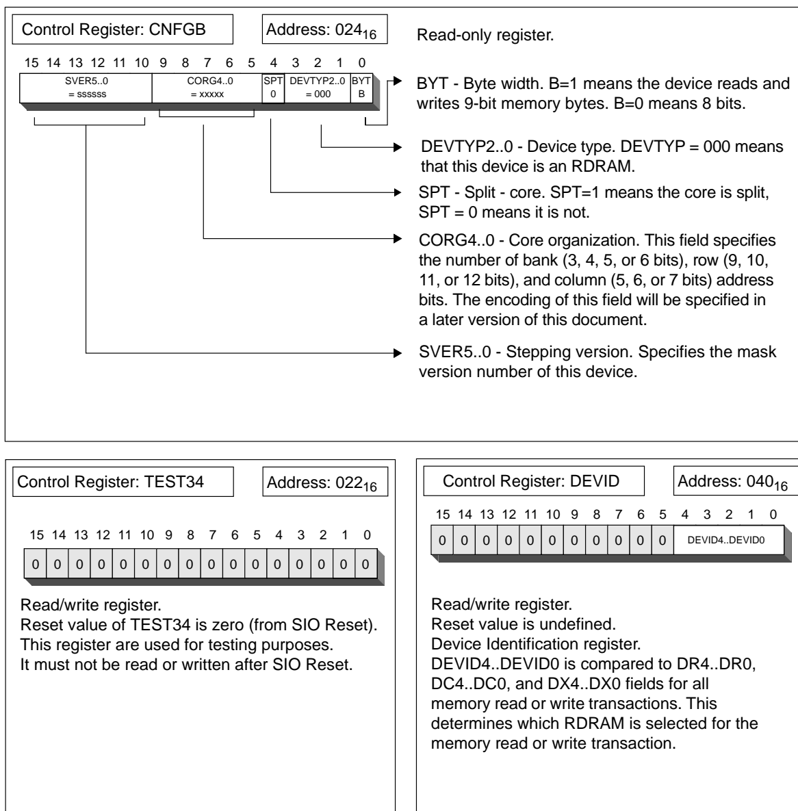
Figure 22-1 Control Registers (2/6)
