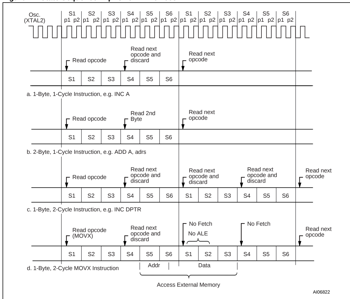
Figure 14. State Sequence in μPSD321X Devices
