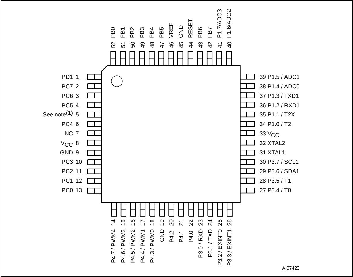
Figure 3. TQFP52 Connections
