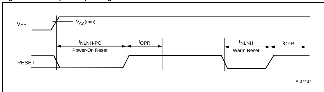
Figure 61. Reset (RESET) Timing
