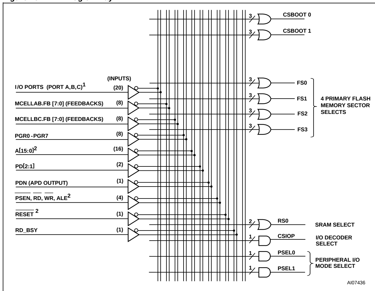
Figure 49. DPLD Logic Array
