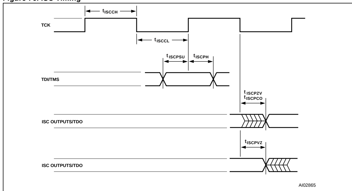
Figure 76. ISC Timing
