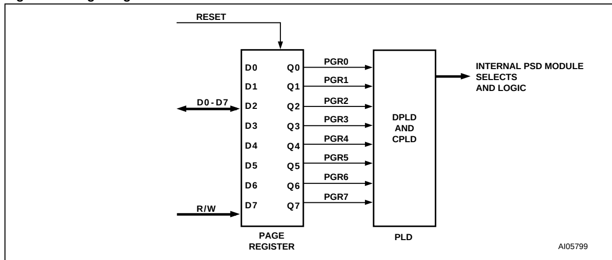
Figure 47. Page Register
