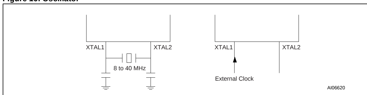
Figure 19. Oscillator
