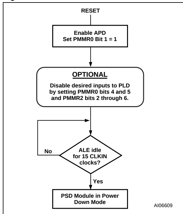
Figure 60. Enable Power-down Flow Chart
