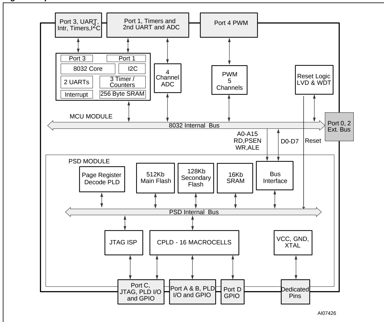
Figure 15. μPSD321X Devices Functional Modules
