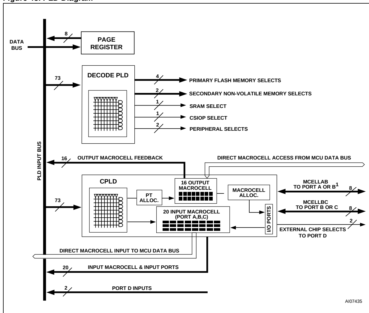
Figure 48. PLD Diagram
