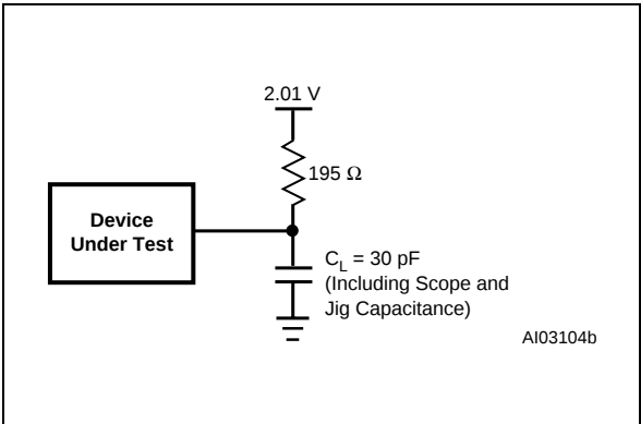
Figure 82. PSD MODULE AC Measurement Load Circuit
