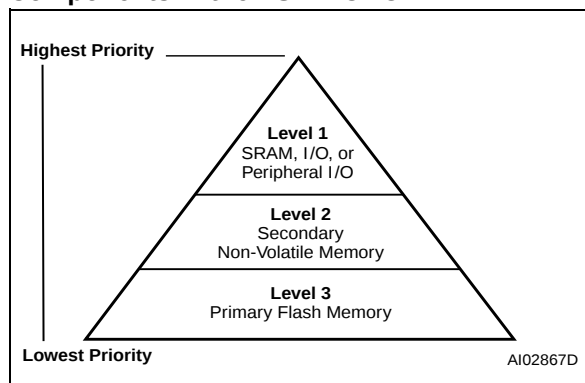
Figure 44. Priority Level of Memory and I/O Components in the PSD MODULE
