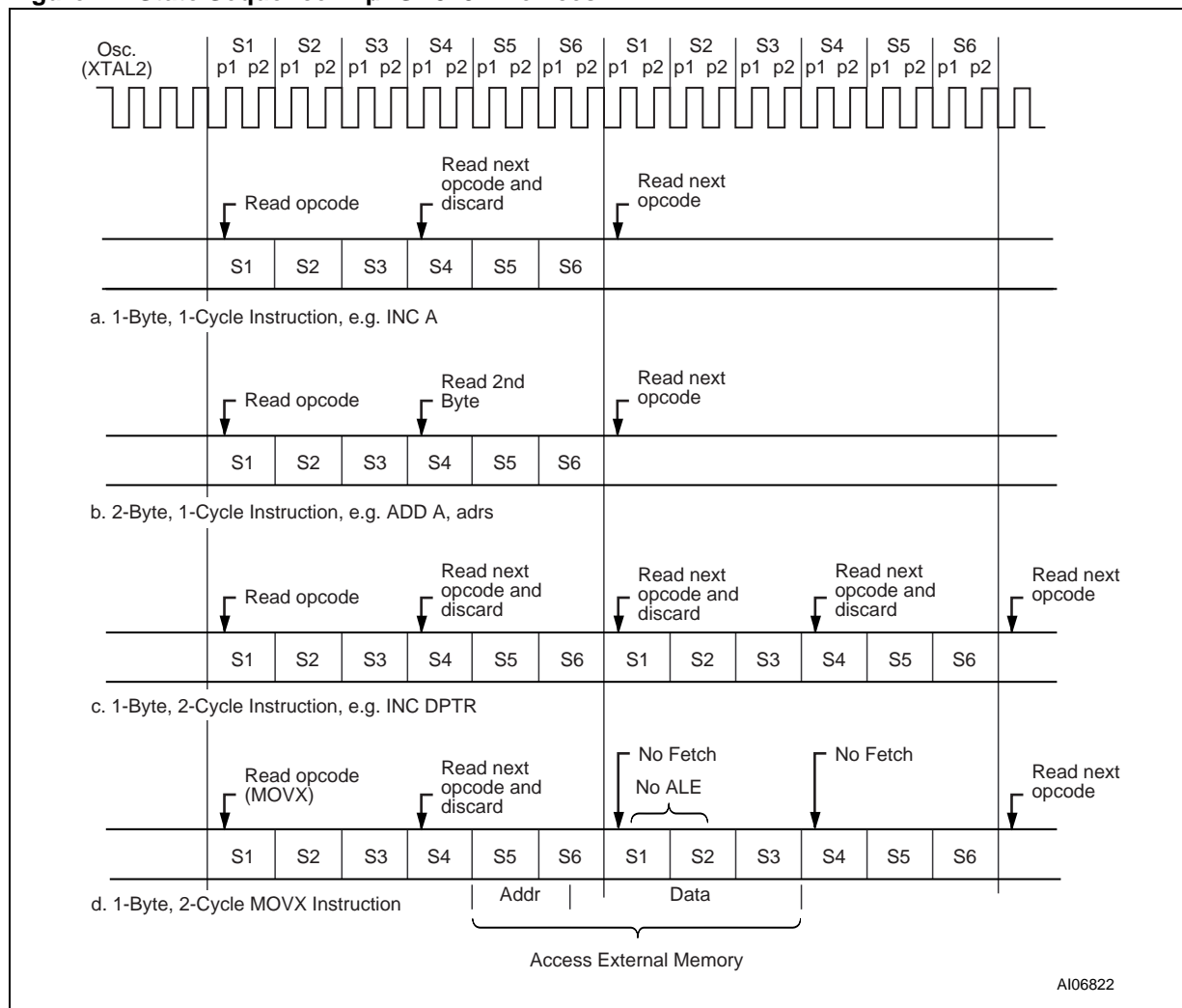
Figure 14. State Sequence in \mu PSD323X Devices
