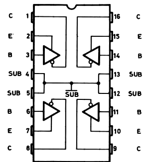
ULN2074B ULN2076B
