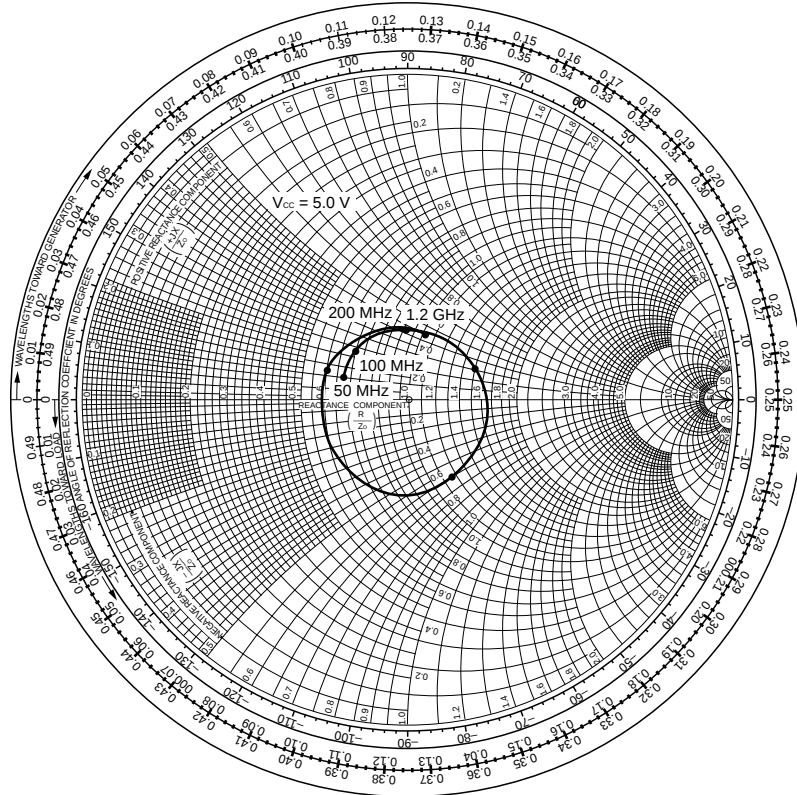
Figure 18 (d). S_{22} vs. f Characteristics of \mu PC1676G
