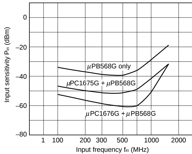
Figure 21. Input Sensitivity Characteristics of \mu PC1675G/1676G + Prescaler \mu PB568G
