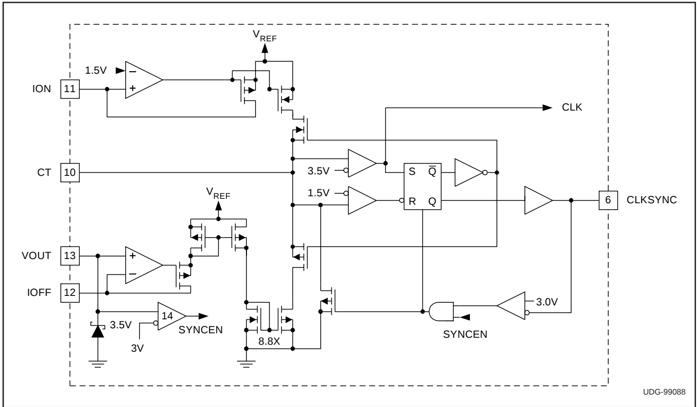
Figure 1. UCC3884 oscillator.
