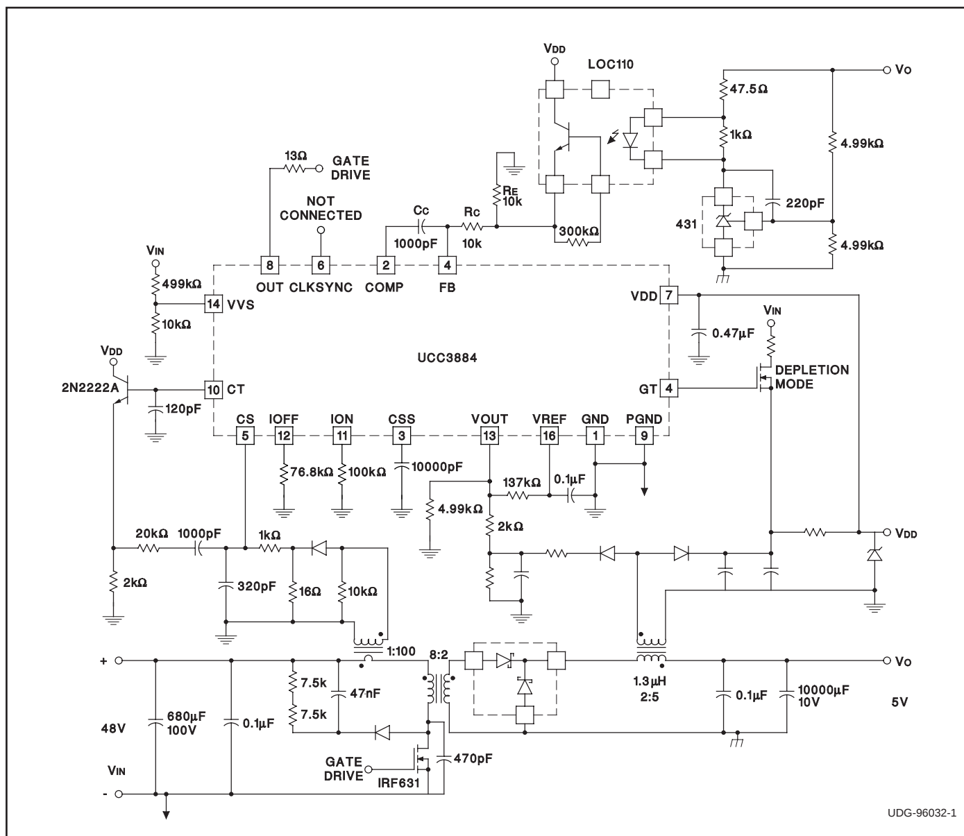
Figure 4. Typical application.
