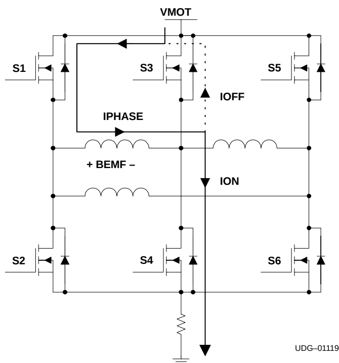
Figure 9. Two-Quadrant Chopping
