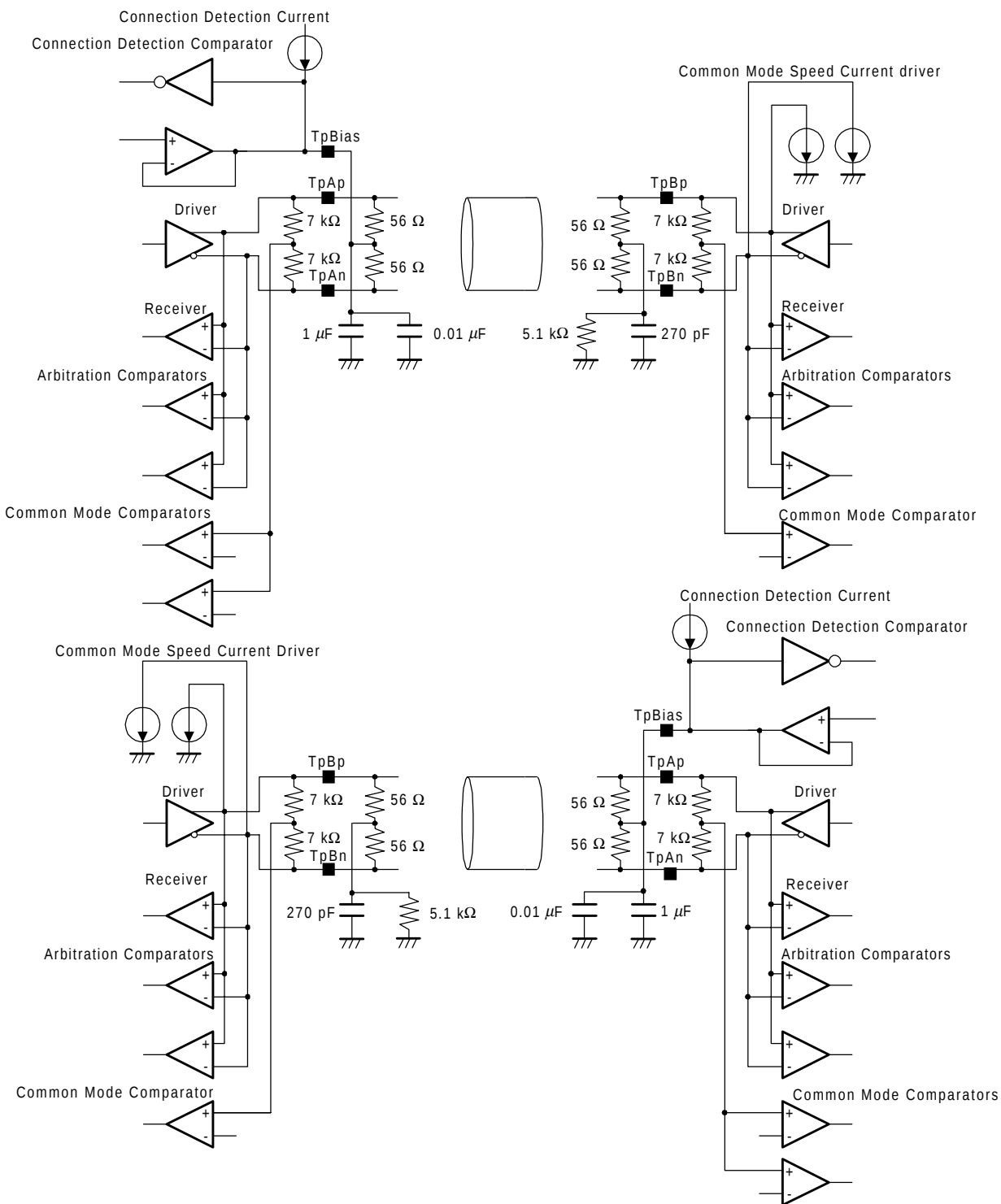
Figure 3-4. Cable Interface
