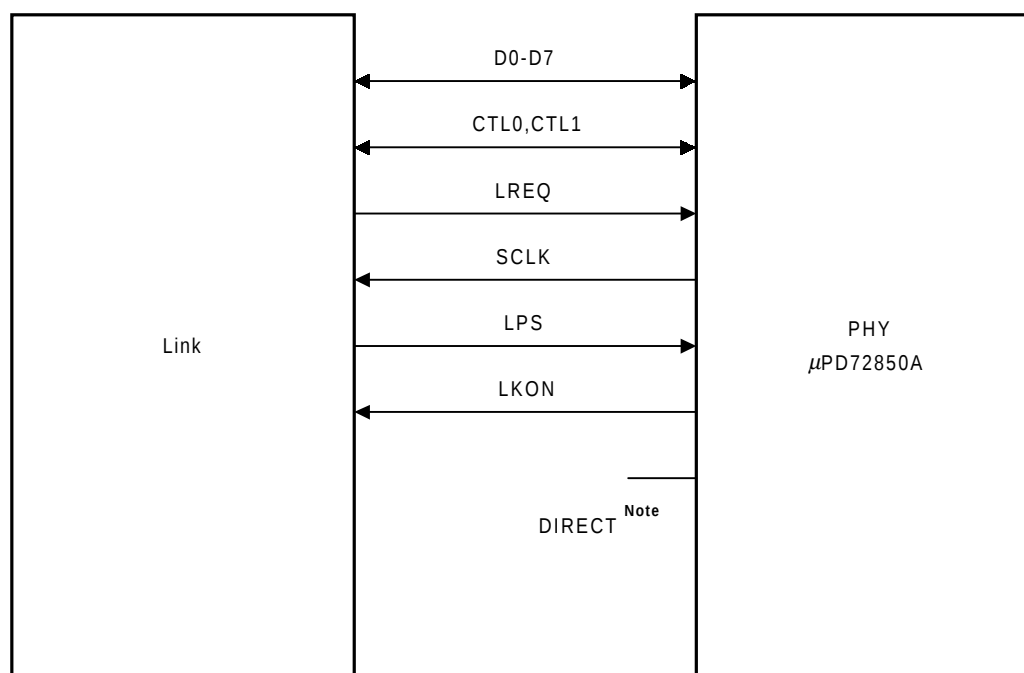
Figure 3-1. PHY/Link Connection Method
