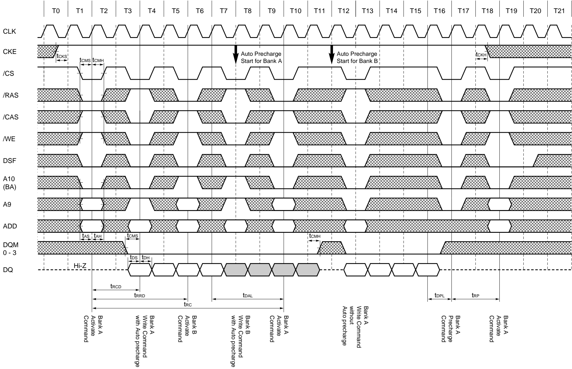
AC Parameters for Write Timing (Burst length = 4, /CAS latency = 2)
