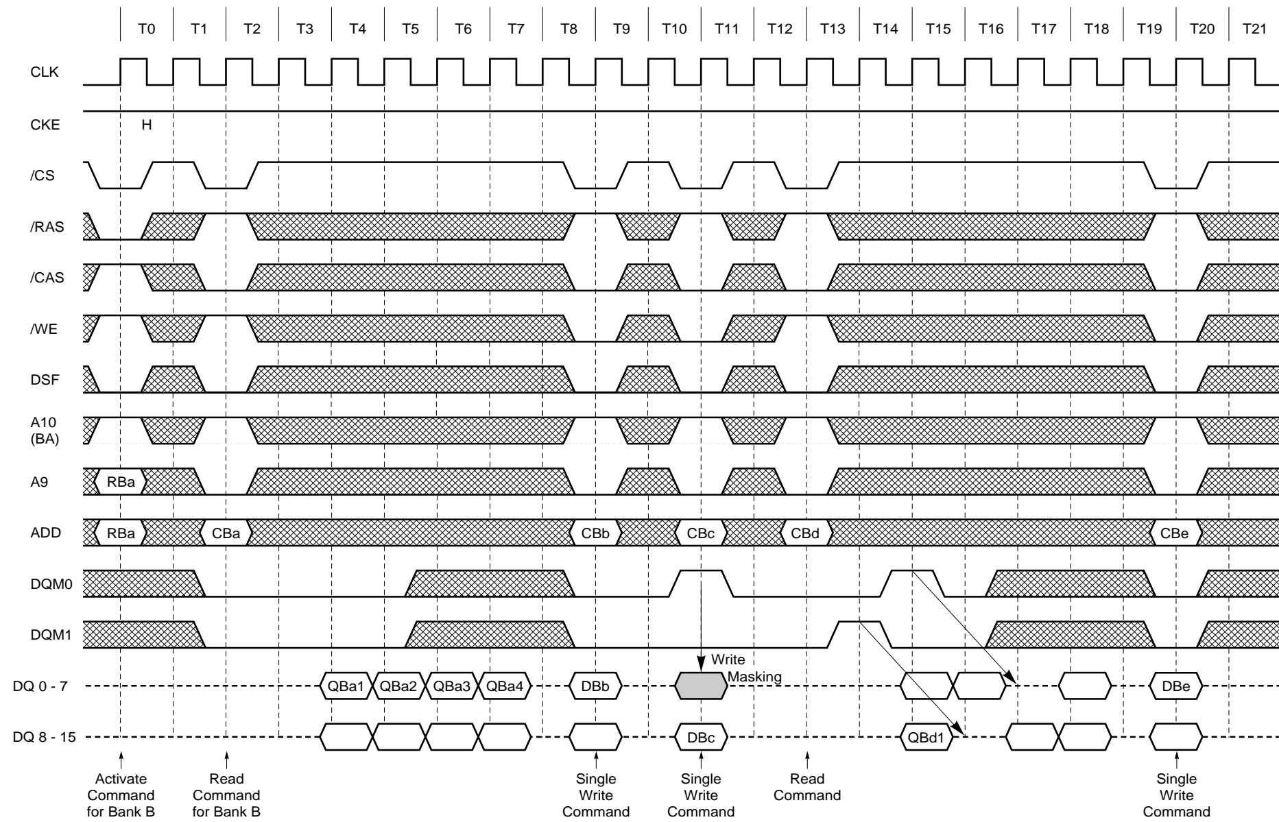
Burst Read and Single Write (Burst length = 4, /CAS latency = 2)
