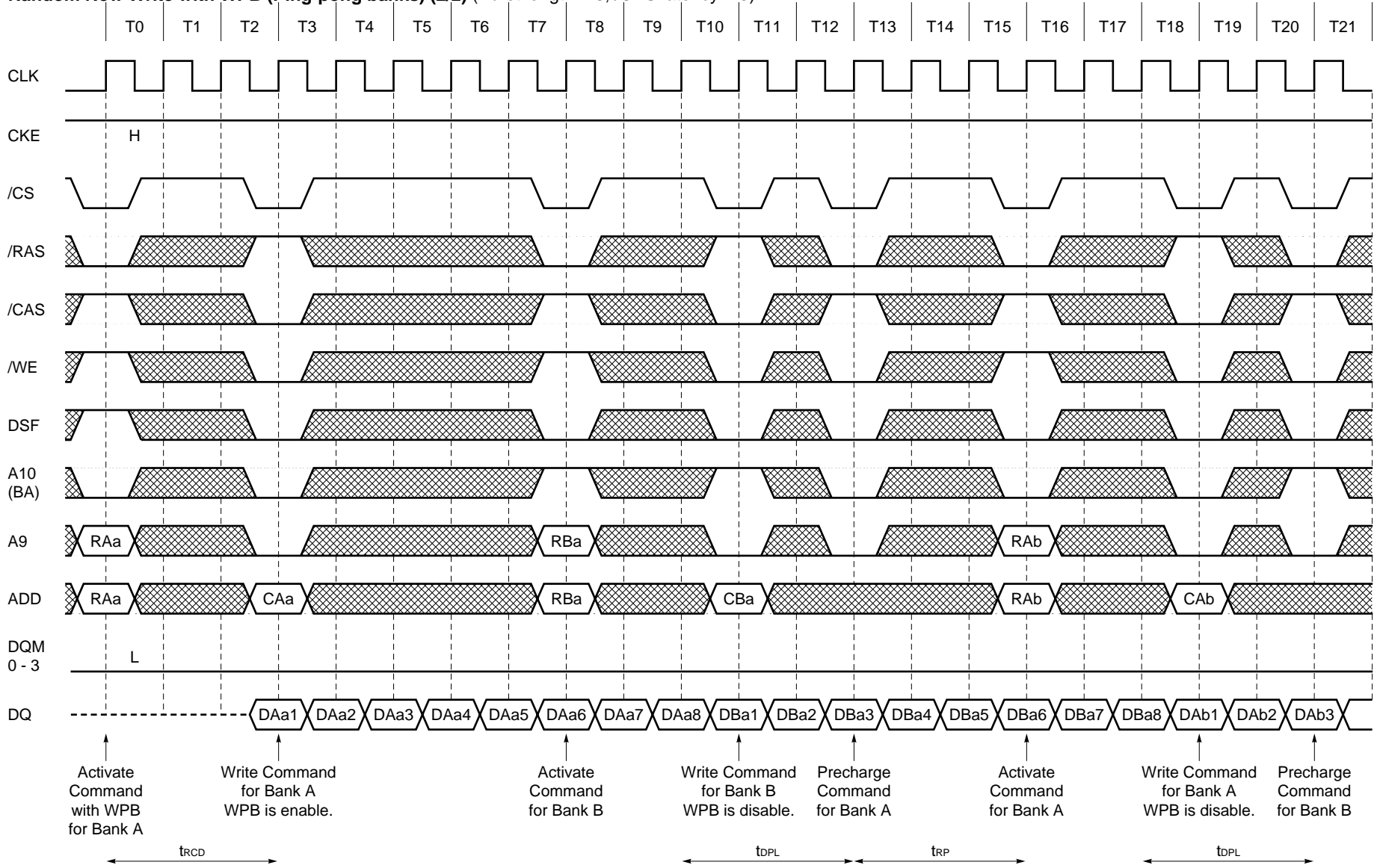
Random Row Write with WPB (Ping-pong banks) (2/2) (Burst length = 8, /CAS latency = 3)
