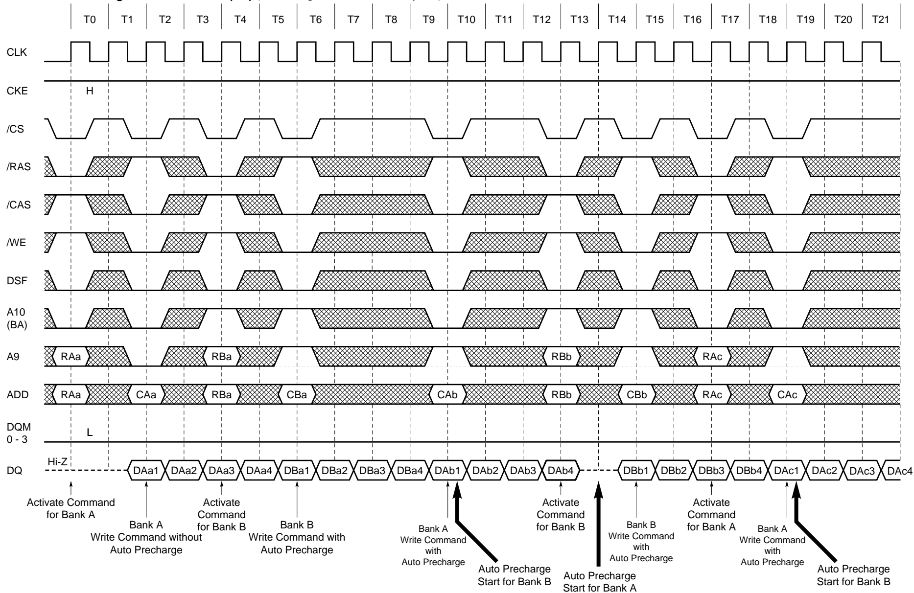
Auto Precharge after Write Burst (1/2) (Burst length = 4, /CAS latency = 2)
