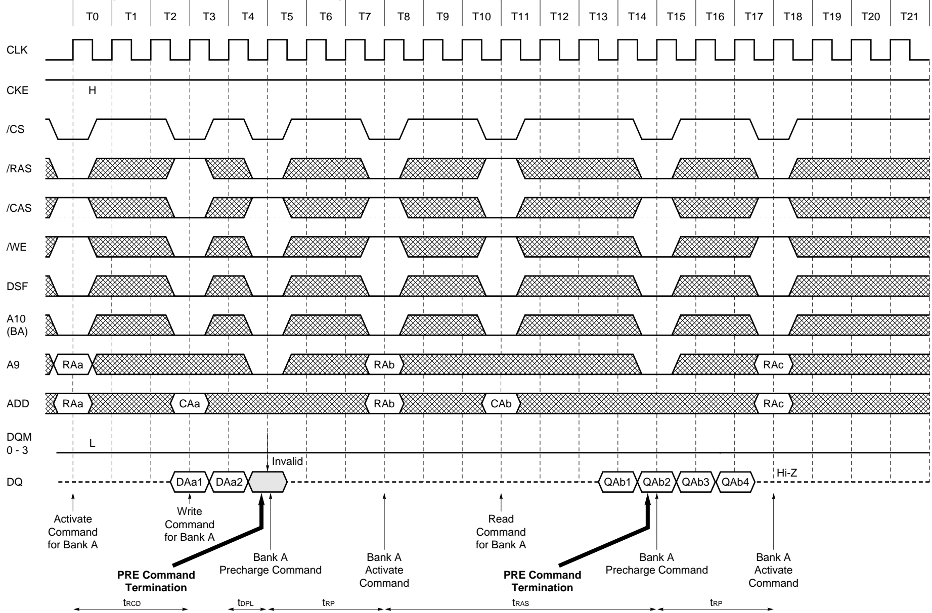
PRE (Precharge) Termination of Burst (2/2) (Burst length = 2, 4, 8, Full, /CAS latency = 3)
