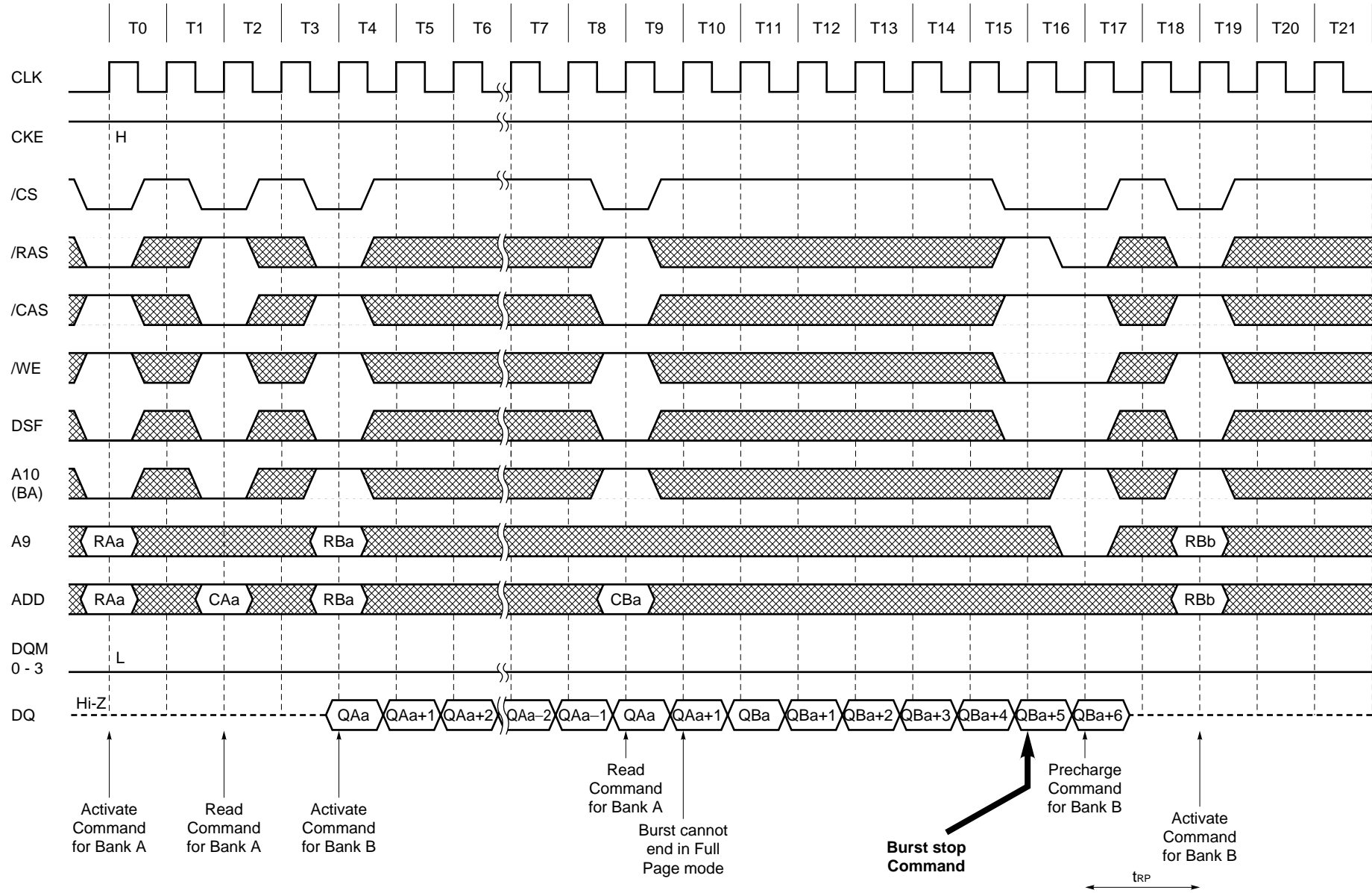
Full Page READ Cycle (1/2) (/CAS latency = 2)
