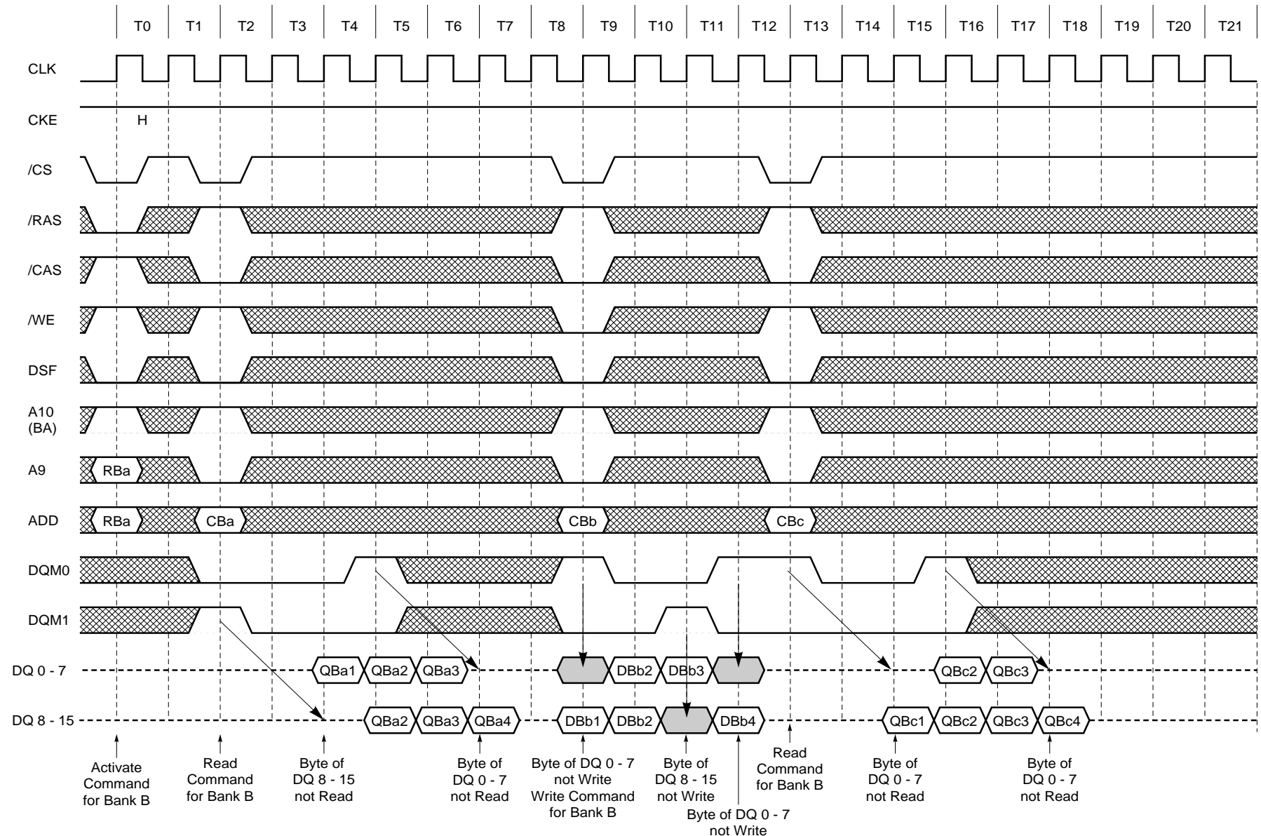
Byte Read/Write Operation (By DQM) (Burst length = 4, /CAS latency = 2)
