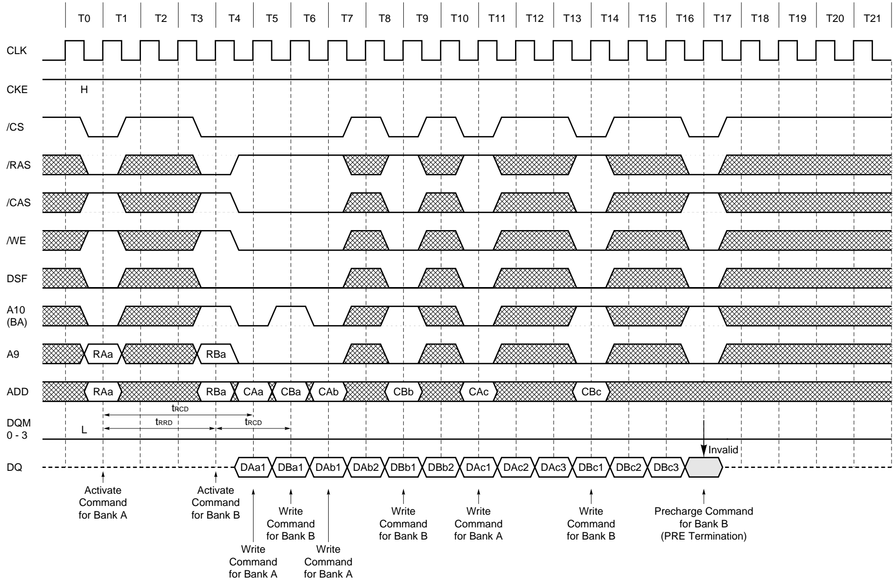
Full Page Random Column Write (Burst length = Full Page, /CAS latency = 2)
