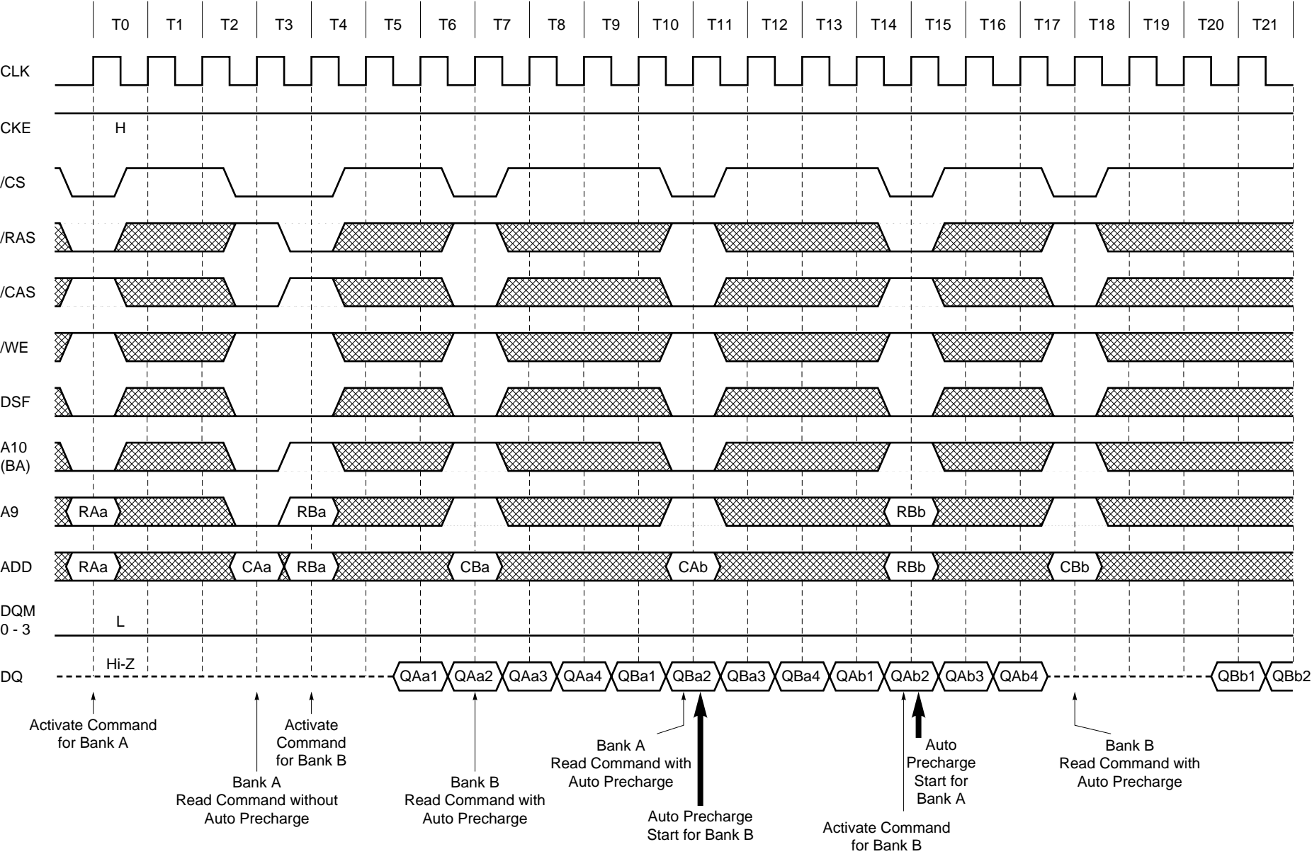
Auto Precharge after Read Burst (2/2) (Burst length = 4, /CAS latency = 3)
