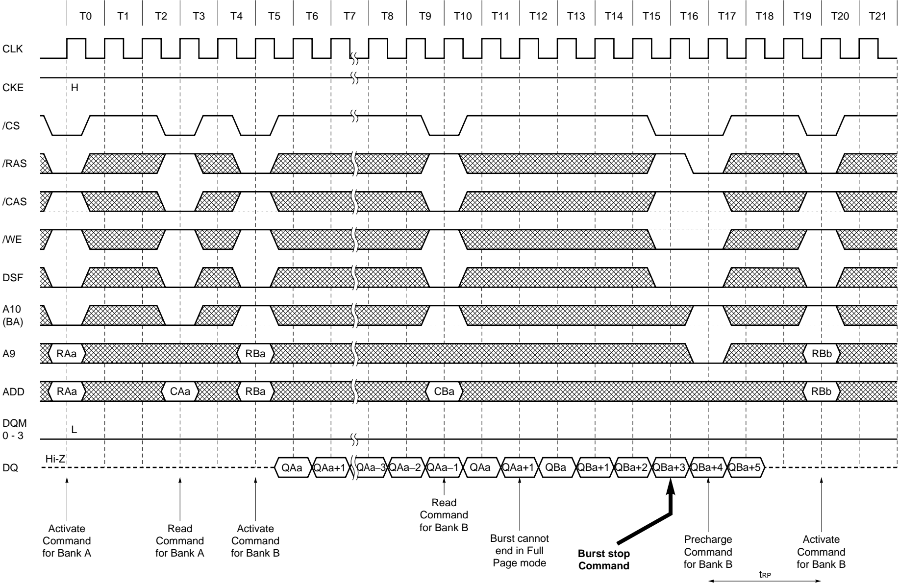
Full Page READ Cycle (2/2) (/CAS latency = 3)
