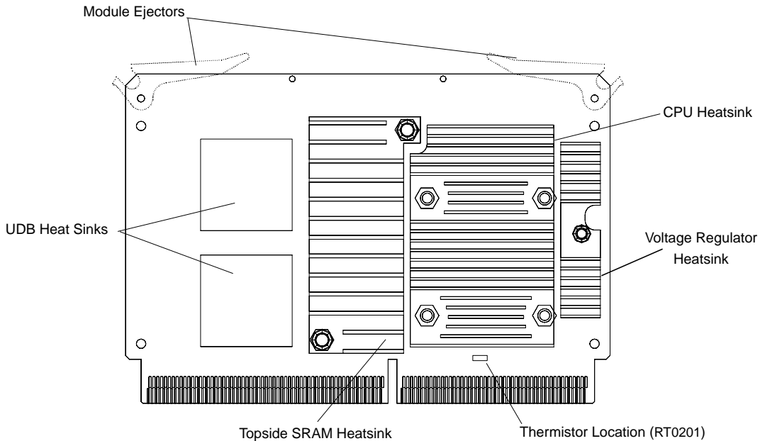
Figure 6. CPU Module (Components)
