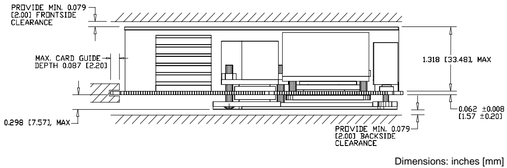
Figure 9. CPU Module Side View with Dimensions
