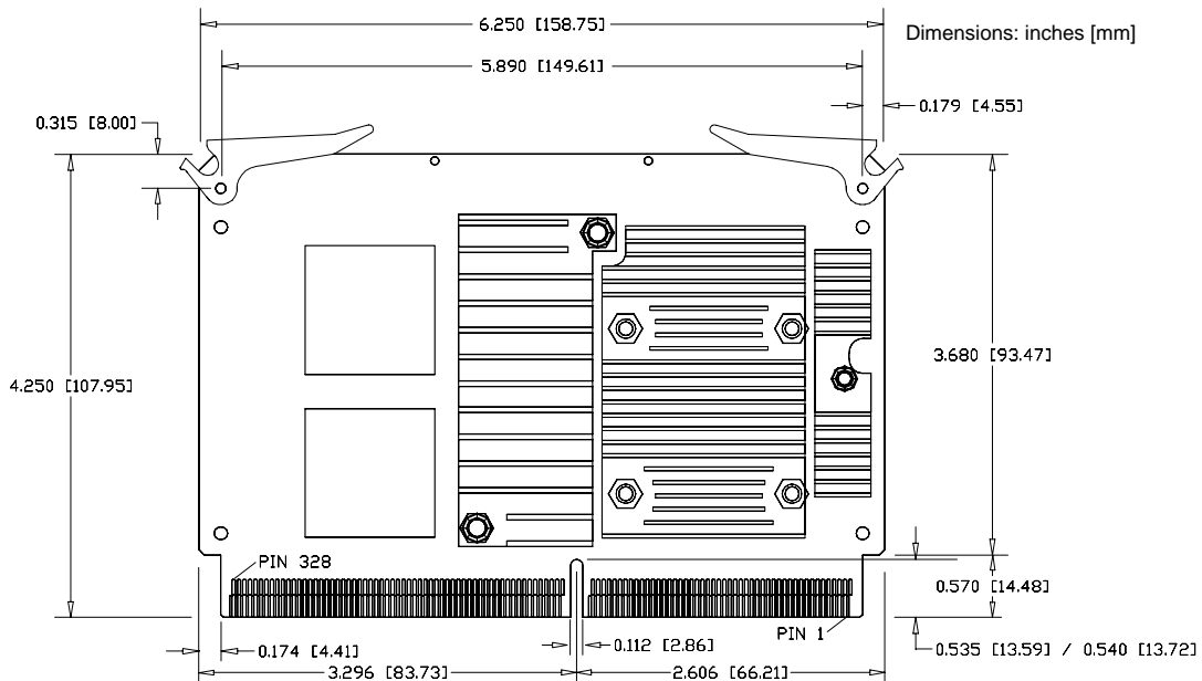
Figure 7. CPU Module (Component Dimensions)
