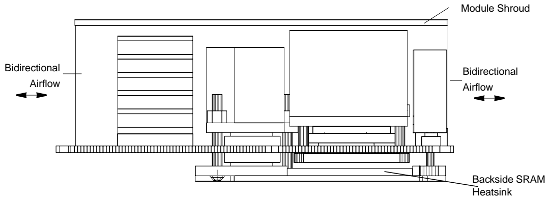
Figure 8. CPU Module Side View
