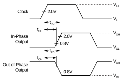
Figure 10. Voltage Waveforms - Propagation Delay Times
