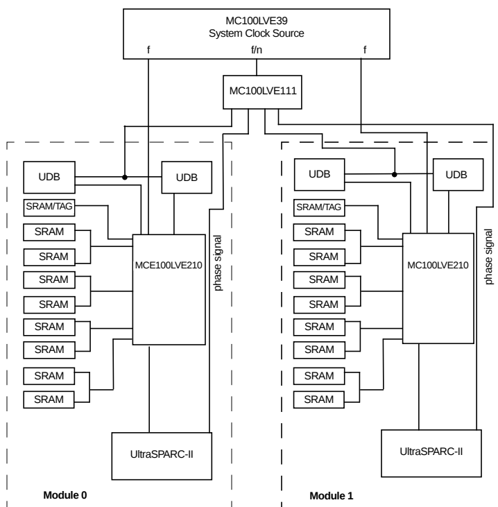
Figure 5. Module Clock Distribution
