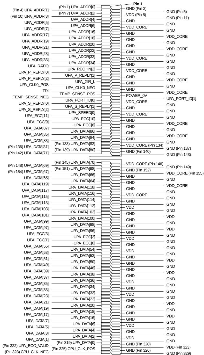
Figure 3. UPA Connector Pin-Out Assignment (Top)
