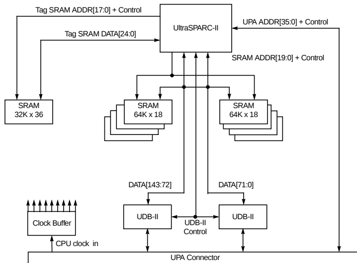
Figure 1. Module Block Diagram
