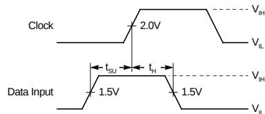
Figure 9. Voltage Waveforms - Setup and Hold Times
