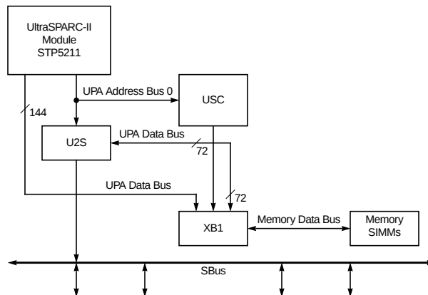
Figure 2. UPA Uniprocessor System Configuration
