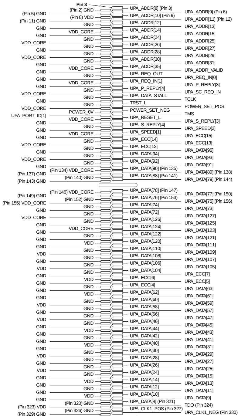
Figure 4. UPA Connector Pin-Out Assignment (Bottom)
