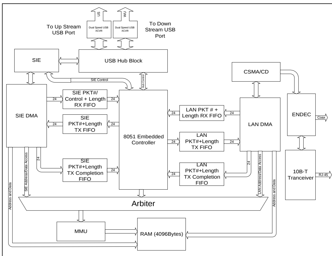
FIGURE 1 – USB97C196 BLOCK DIAGRAM
