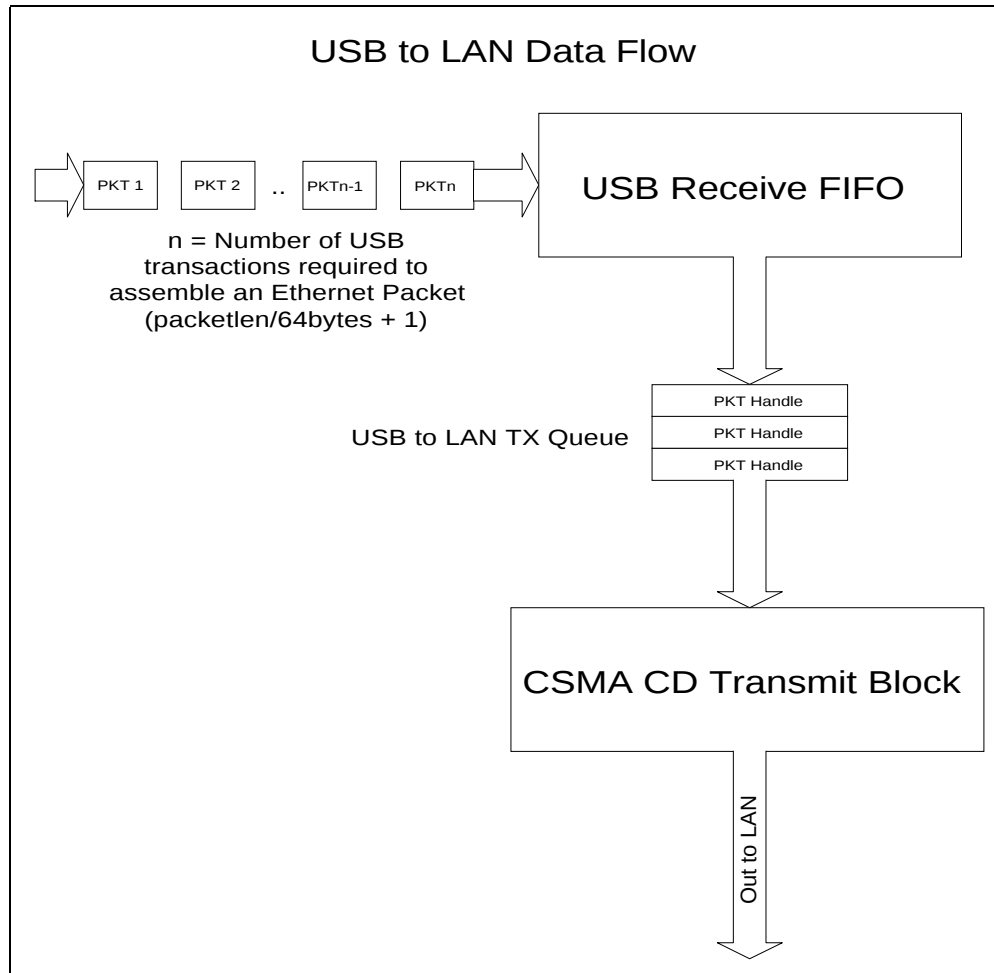
FIGURE 2 – USB TO LAN DATA FLOW
