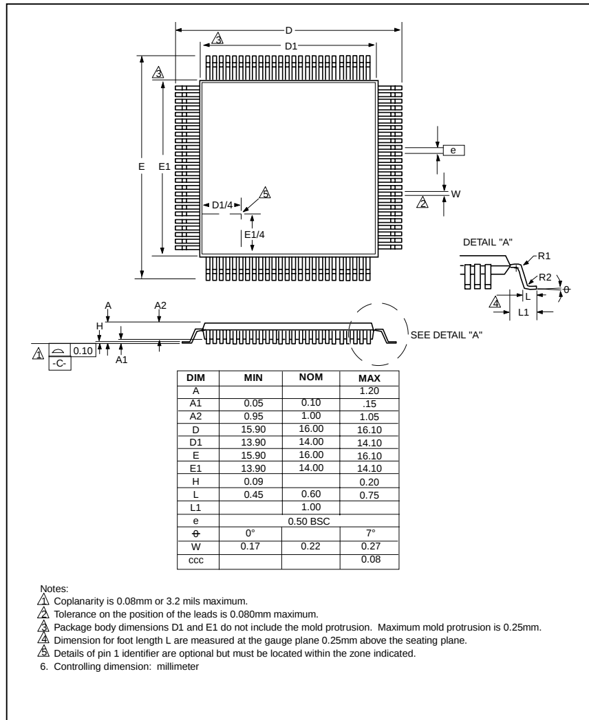
FIGURE 16 – 100 PIN TQFP PACKAGE OUTLINE
