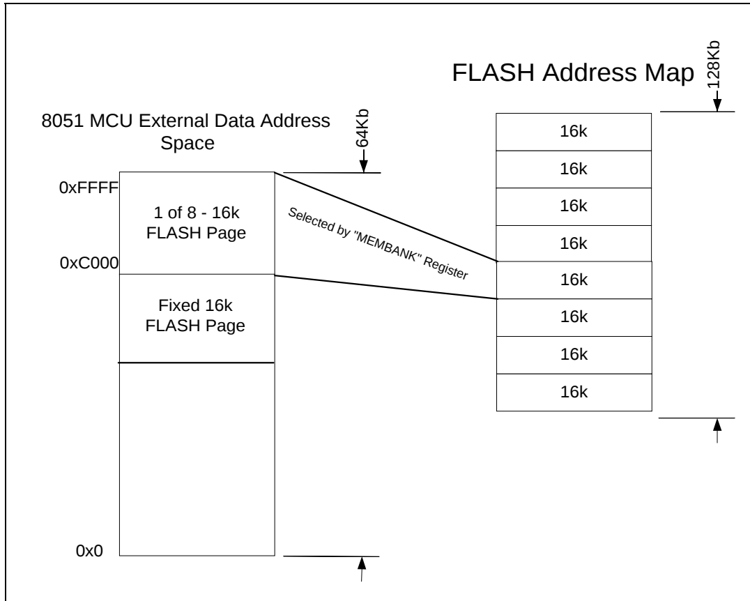
FIGURE 7 - MCU TO EXTERNAL DATA MEMORY MAP DIAGRAM
