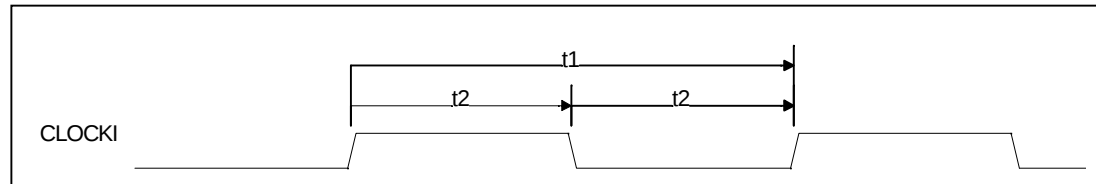
FIGURE 11 – INPUT ETHERNET CLOCK TIMING
