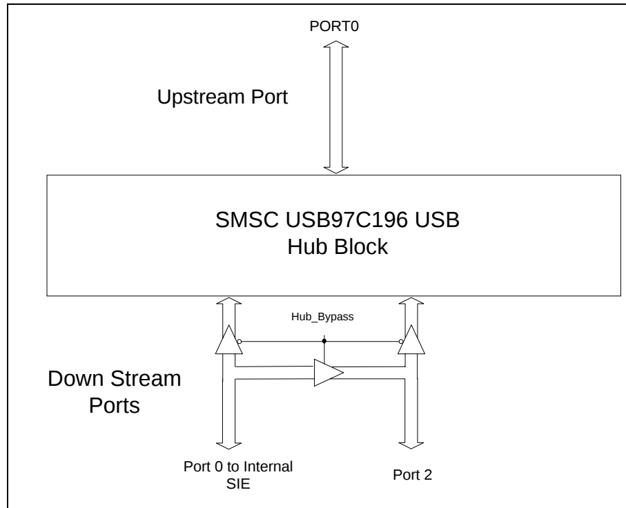
FIGURE 9 - USB97C196 HUB BYPASS MODE
