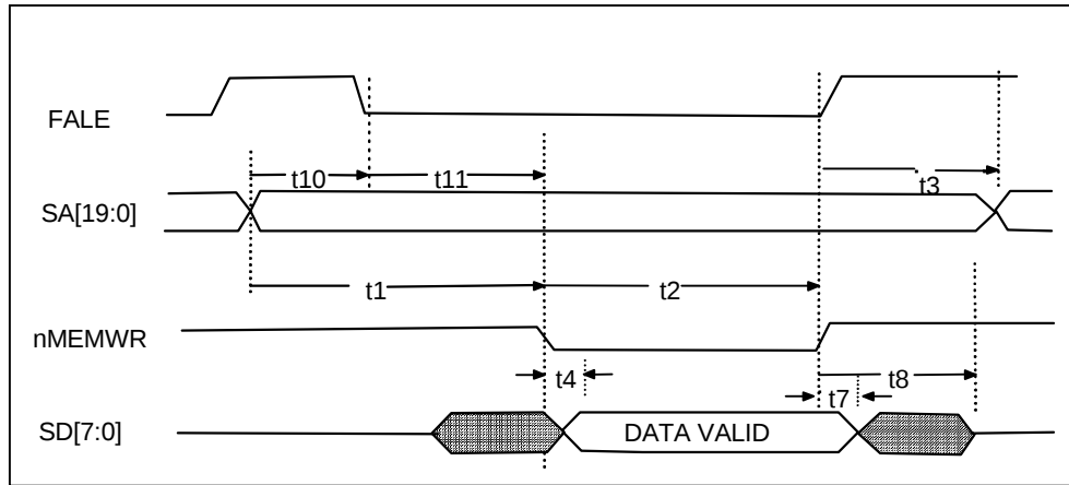
FIGURE 14 - 8051 FLASH MEMORY WRITE TIMING
