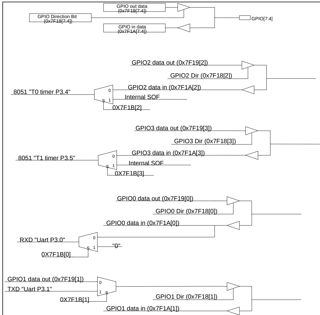
FIGURE 8 - GPIO MUXING BLOCK DIAGRAM
