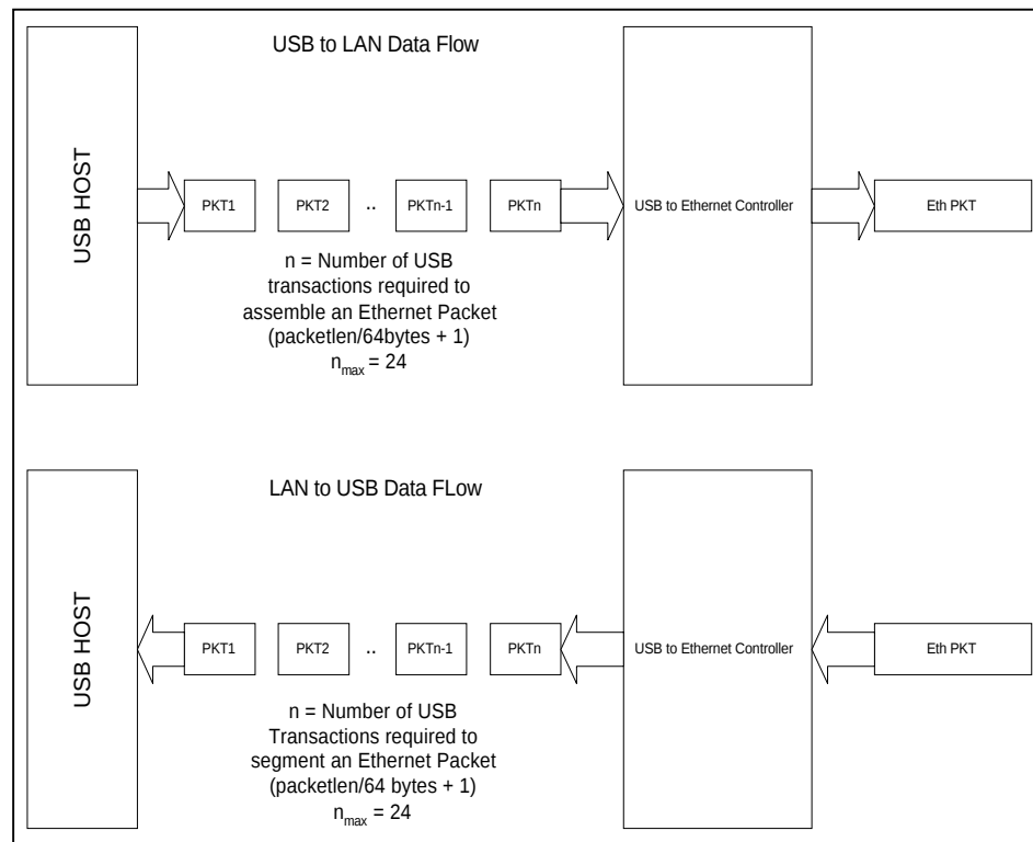
FIGURE 4 - SEGMENTATION AND RE-ASSEMBLY
