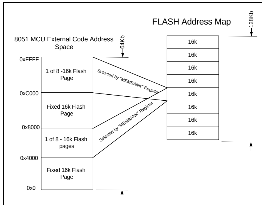
FIGURE 6 - MCU TO EXTERNAL CODE SPACE MAP DIAGRAM
