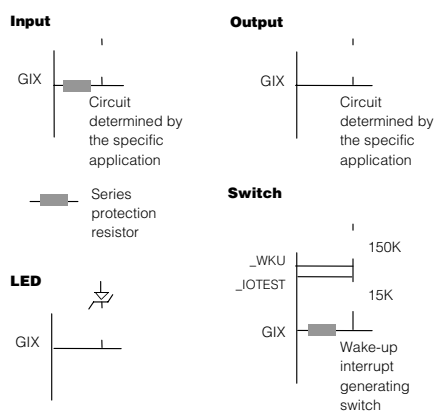
Figure 3: Suggested interface of general purpose input/output pin
