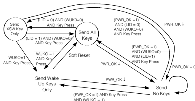
Figure 2: The UR5HCSPI-SA implements four modes of keyboard and switch operation.
