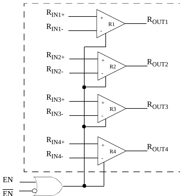
Figure 1. UT54LVDSC032 Quad Receiver Block Diagram
