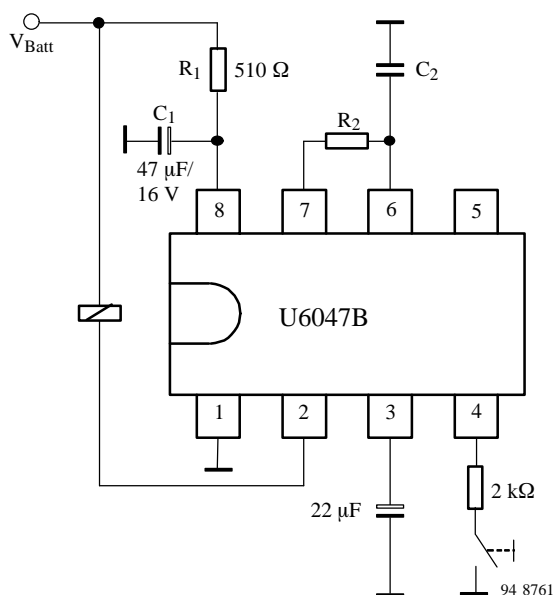
Figure 13. Generation of a monostable delay time, t_d , by applying the operating voltage V_{Batt} , deactivatable by the OFF push-button
