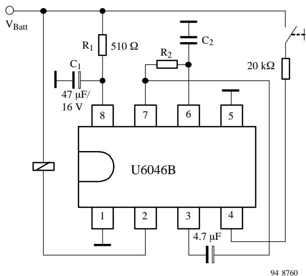
Figure 13. Generation of a monostable delay time, t_d , by applying the operating voltage V_{Batt} , deactivatable by the OFF push-button
