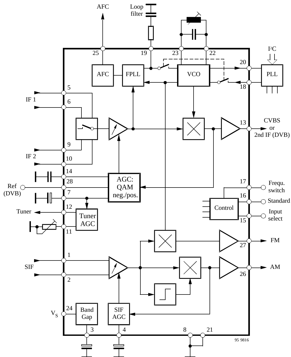
Figure 1. Block diagram
