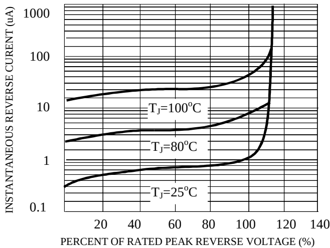
FIG. 3-TYPICAL REVERSE CHARACTERISTICS
