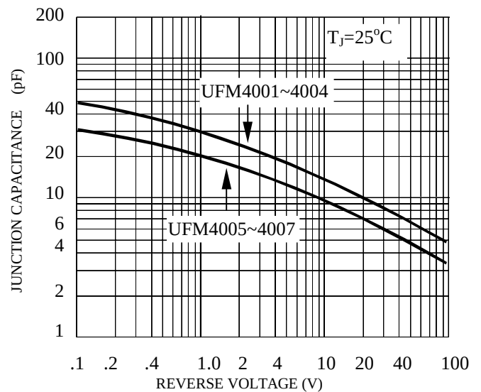
FIG. 6-TYPICAL JUNCTION CAPACITANCE
