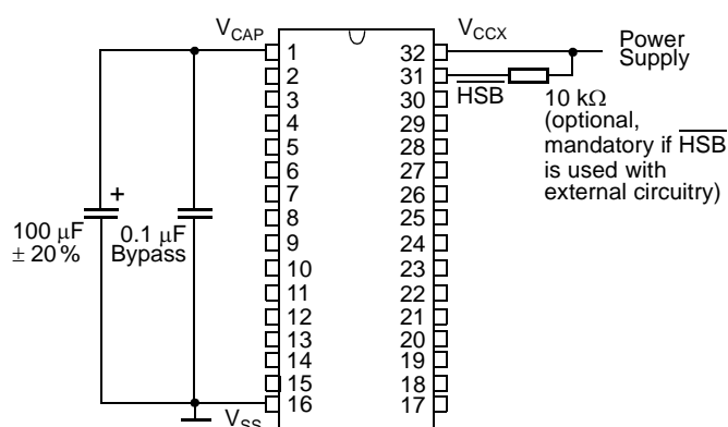
Figure 1: AUTOMATIC STORE OPERATION Schematic Diagram
