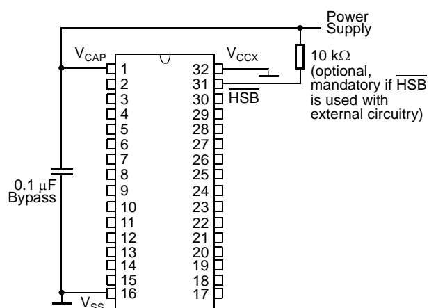
Figure 2: DISABELING AUTOMATIC STORES Schematic Diagram
