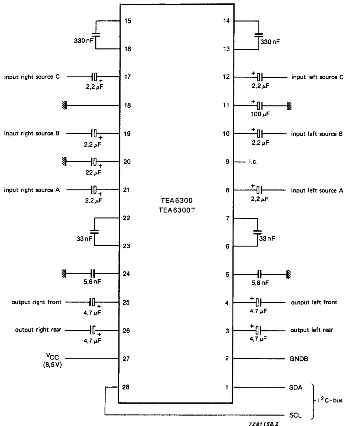
Fig.10 Test and application circuit.
