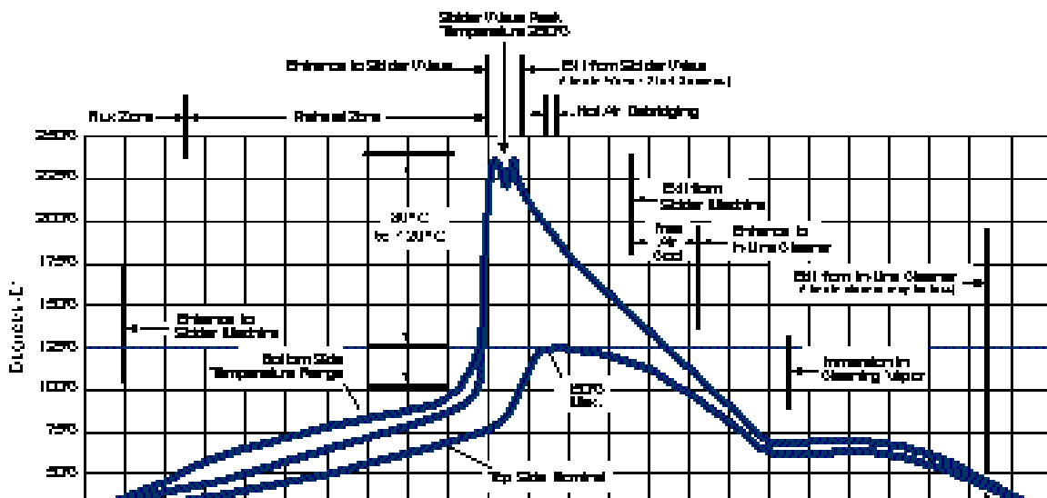
Figure 7. Optimum Solder Wave Profile
