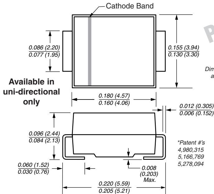
DO-214AA (SMB)
